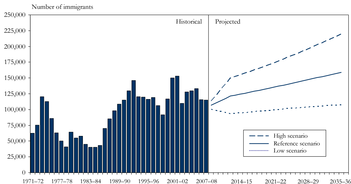
Chart 16 Immigration to Ontario, 1971 to 2036
