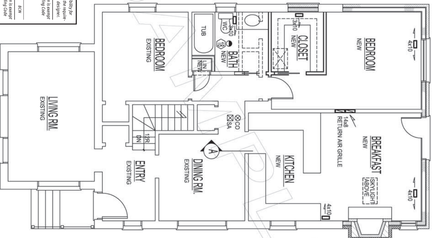
FIRST FLOOR HVAC PLAN SCALE 3/16" = 1'-0"
