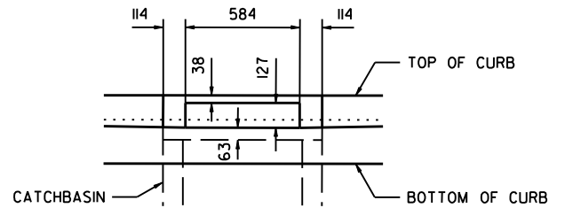
CURB ELEVATION
