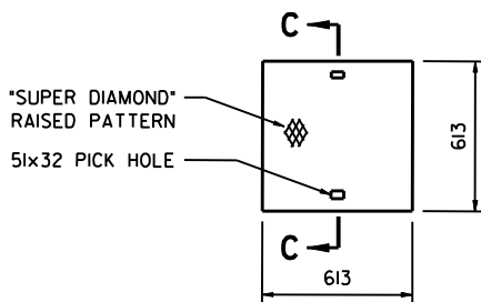
COVER PLAN VIEW
