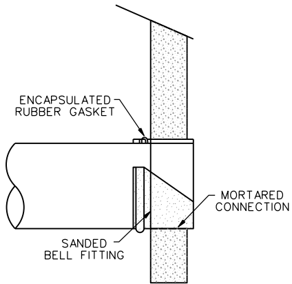
SAND COLLAR
