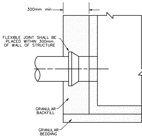
ELEVATION FLEXIBLE JOINT FLEXIBLE PIPE
