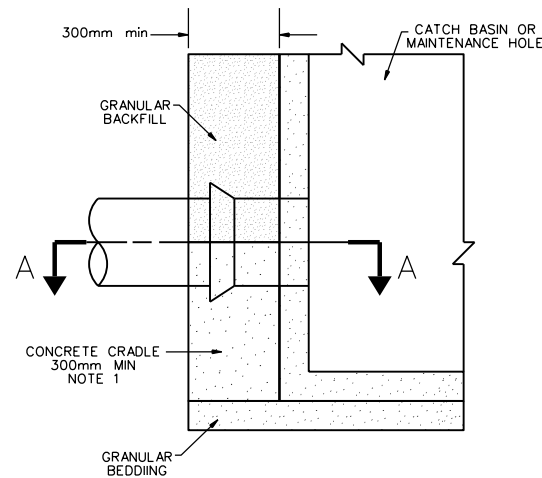
ELEVATION CONCRETE CRADLE RIGID PIPE
