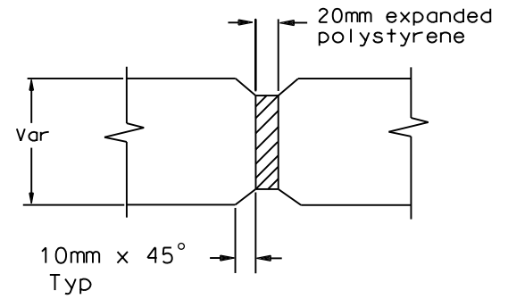
CONTRACTION JOINT IN CONCRETE TOE WALLS
