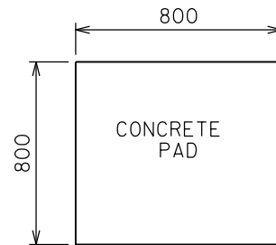
Type "D" Single Concrete Pad
