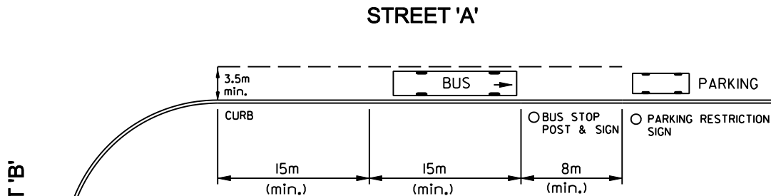
FARSIDE OF INTERSECTION BUS STOP FOR STANDARD 12.2m (40') BUS
