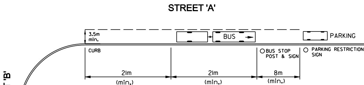
FARSIDE OF INTERSECTION BUS STOP FOR ARTICULATED 18.3m (60') BUS
