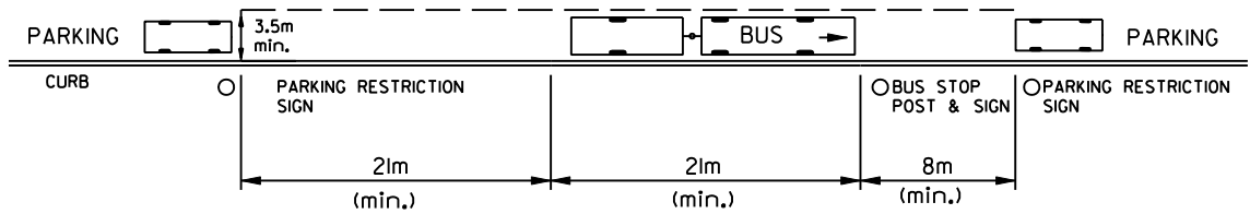
MIDBLOCK OF INTERSECTIONS BUS STOP FOR ARTICULATED 18.3m (60') BUS
