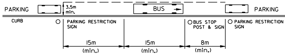
MIDBLOCK OF INTERSECTIONS BUS STOP FOR STANDARD 12.2m (40') BUS
