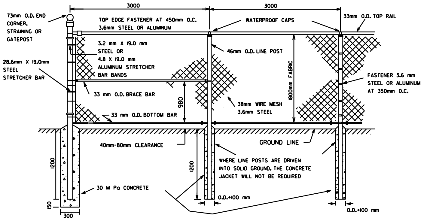
1800 CHAIN LINK FENCE
