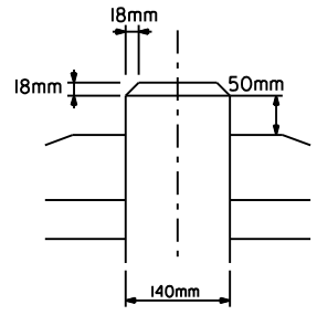
POST DETAIL TYPE 'A'
