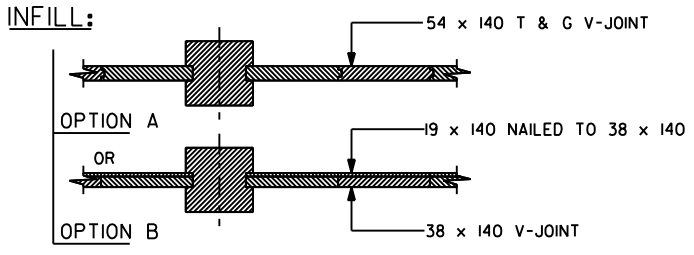
TYPICAL SECTION
