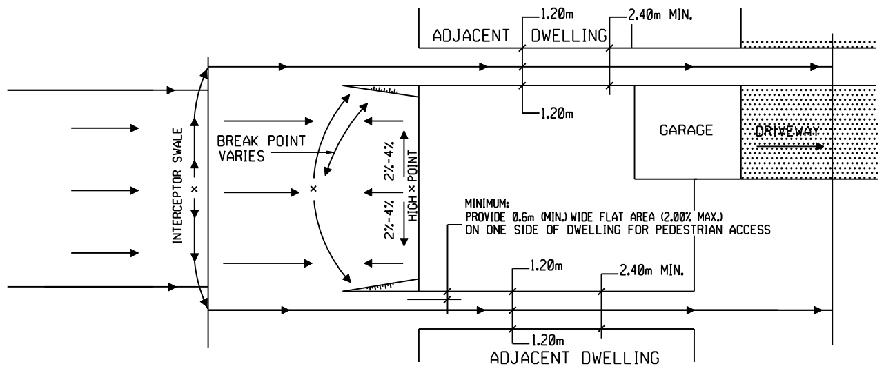
REAR TO FRONT LOT DRAINAGE (FOR LOT FRONTAGES > 12.0m.)
