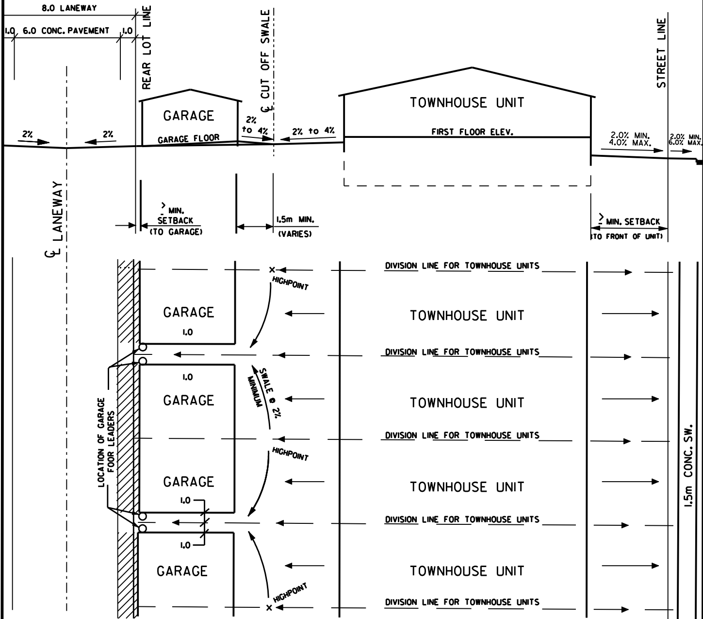
SPLIT LOT DRAINAGE (FOR TOWNHOUSE UNITS BACKING ONTO LANEWAY)
