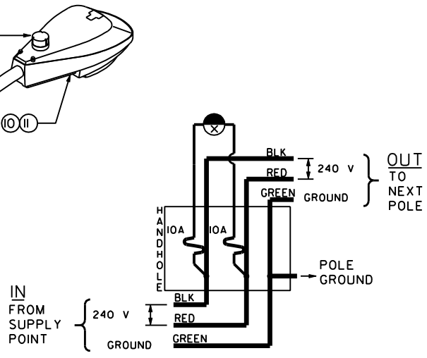
SCHEMATIC DIAGRAM
