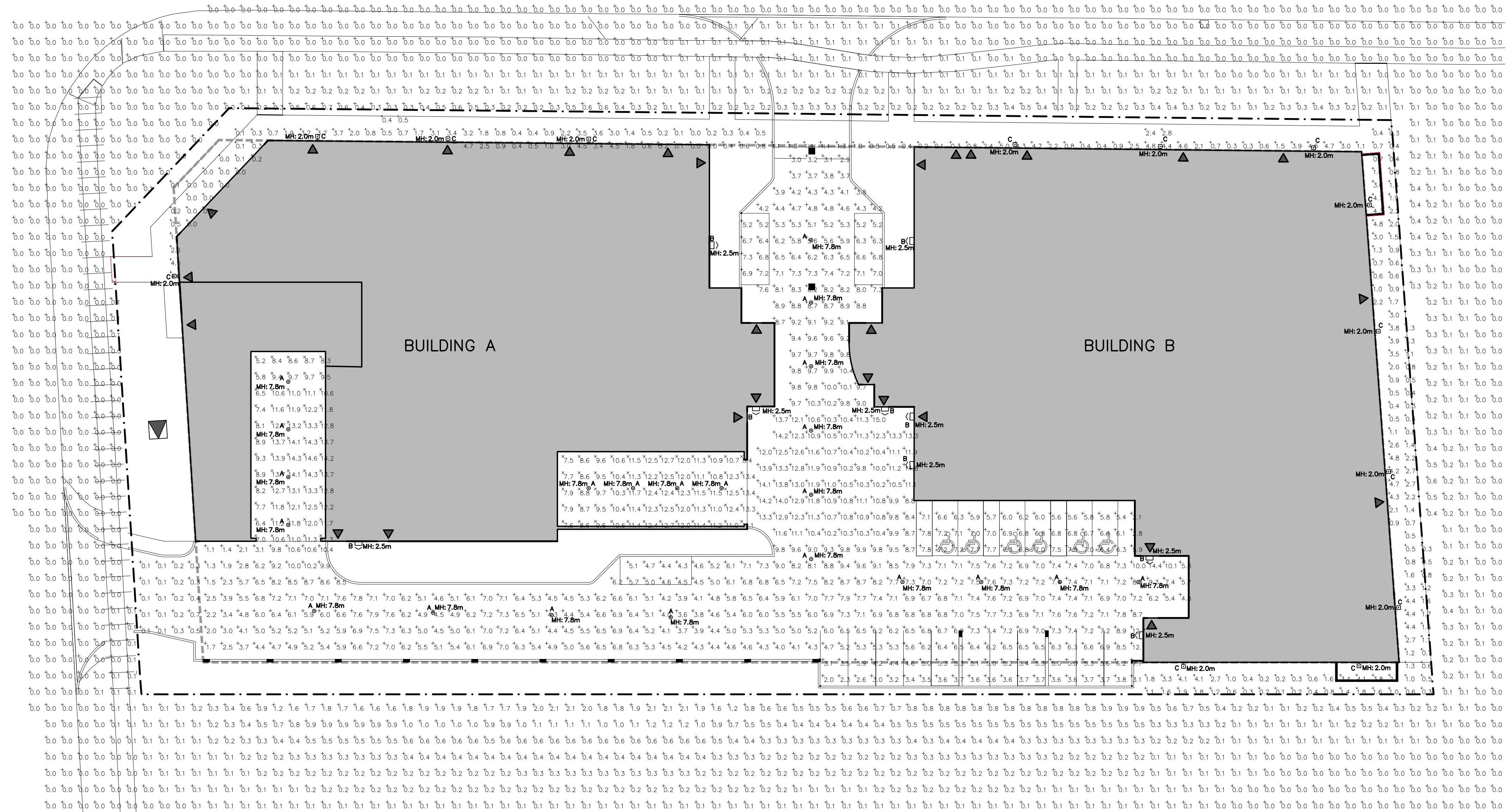
SITE PLAN – PHOTOMETRIC SCALE: 1:250
