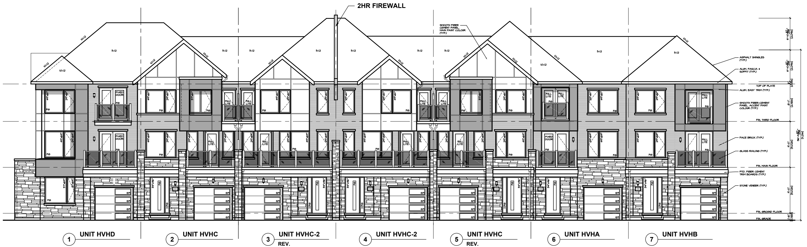
EAST ELEVATION 'MO' VILLAGE HOMES BLOCK 21
