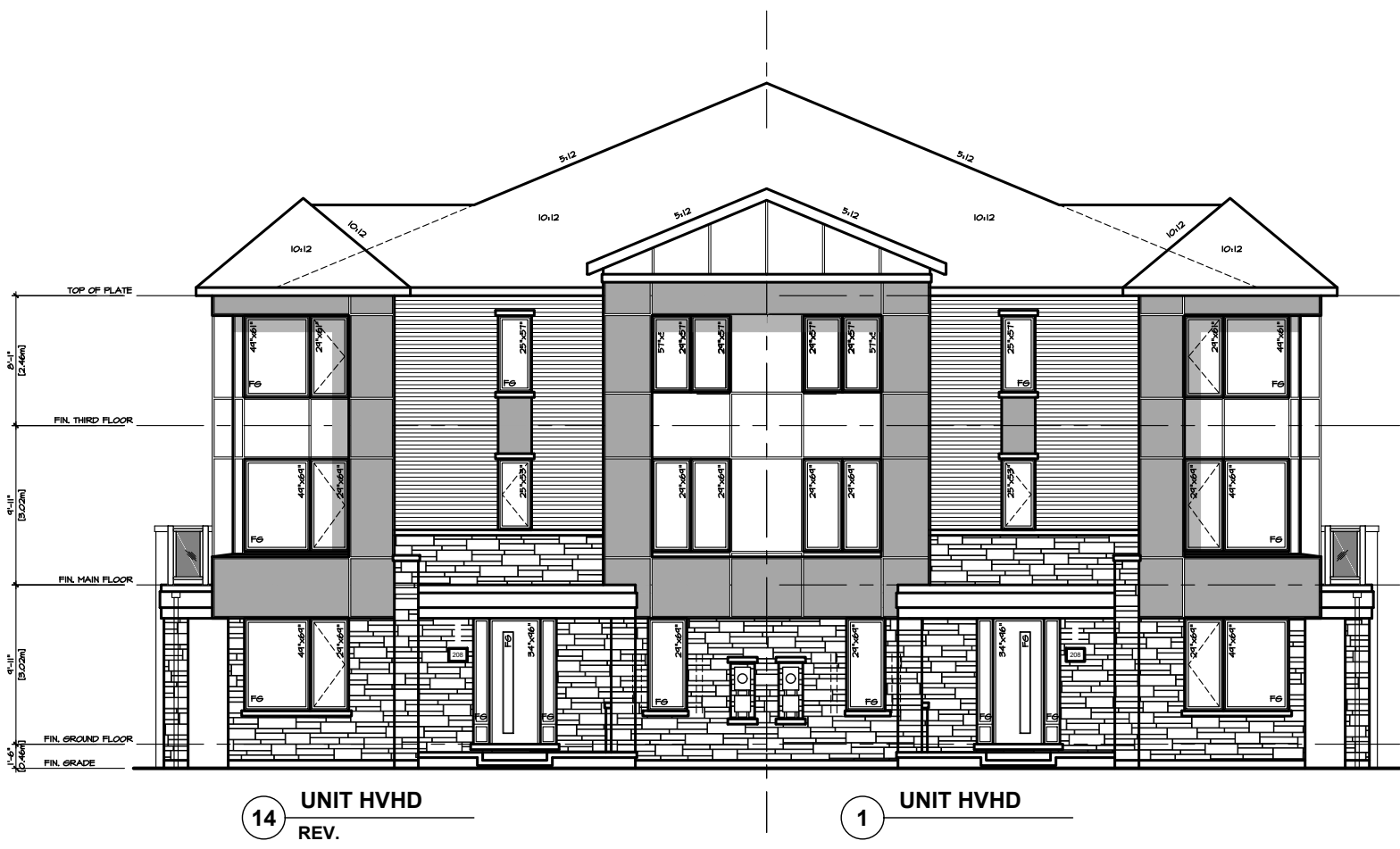
SOUTH SIDE ELEVATION 'MO' VILLAGE HOMES BLOCK 21
