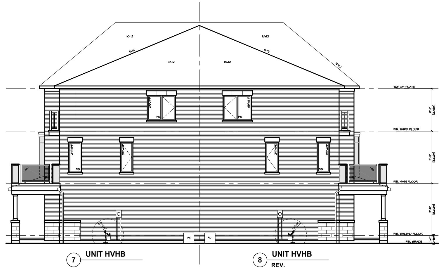
NORTH SIDE ELEVATION 'TA' VILLAGE HOMES BLOCK 22
