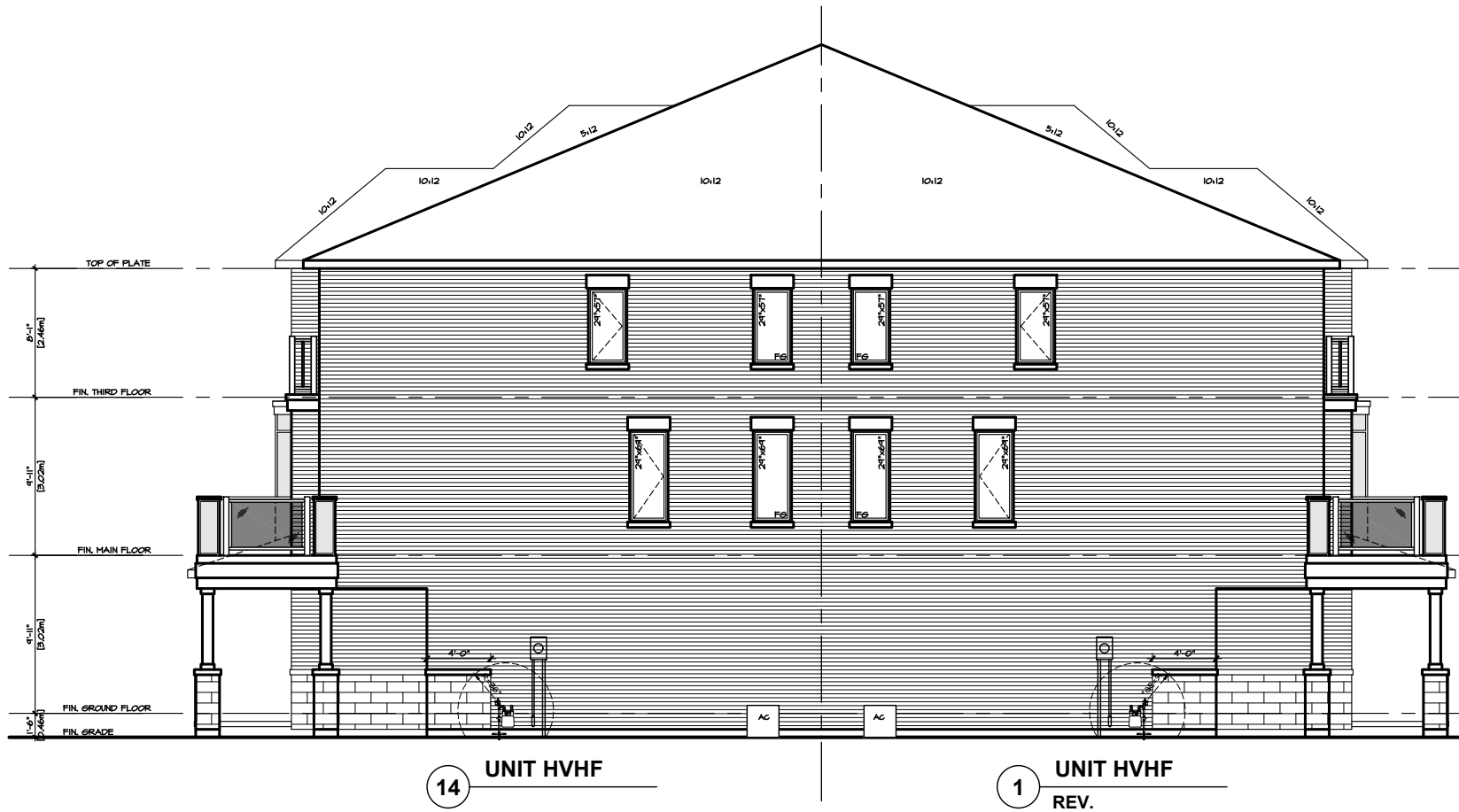
SOUTH SIDE ELEVATION 'TA' VILLAGE HOMES BLOCK 22
