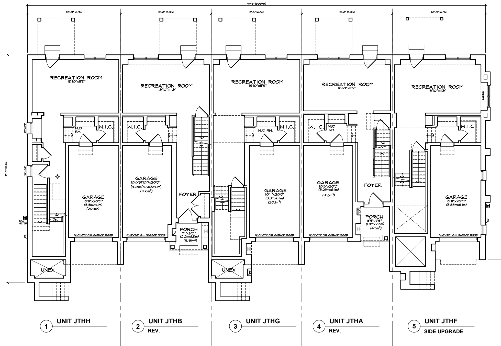
GROUND FLOOR PLAN 'TA' FRONT LOAD TOWNS BLOCK 20
