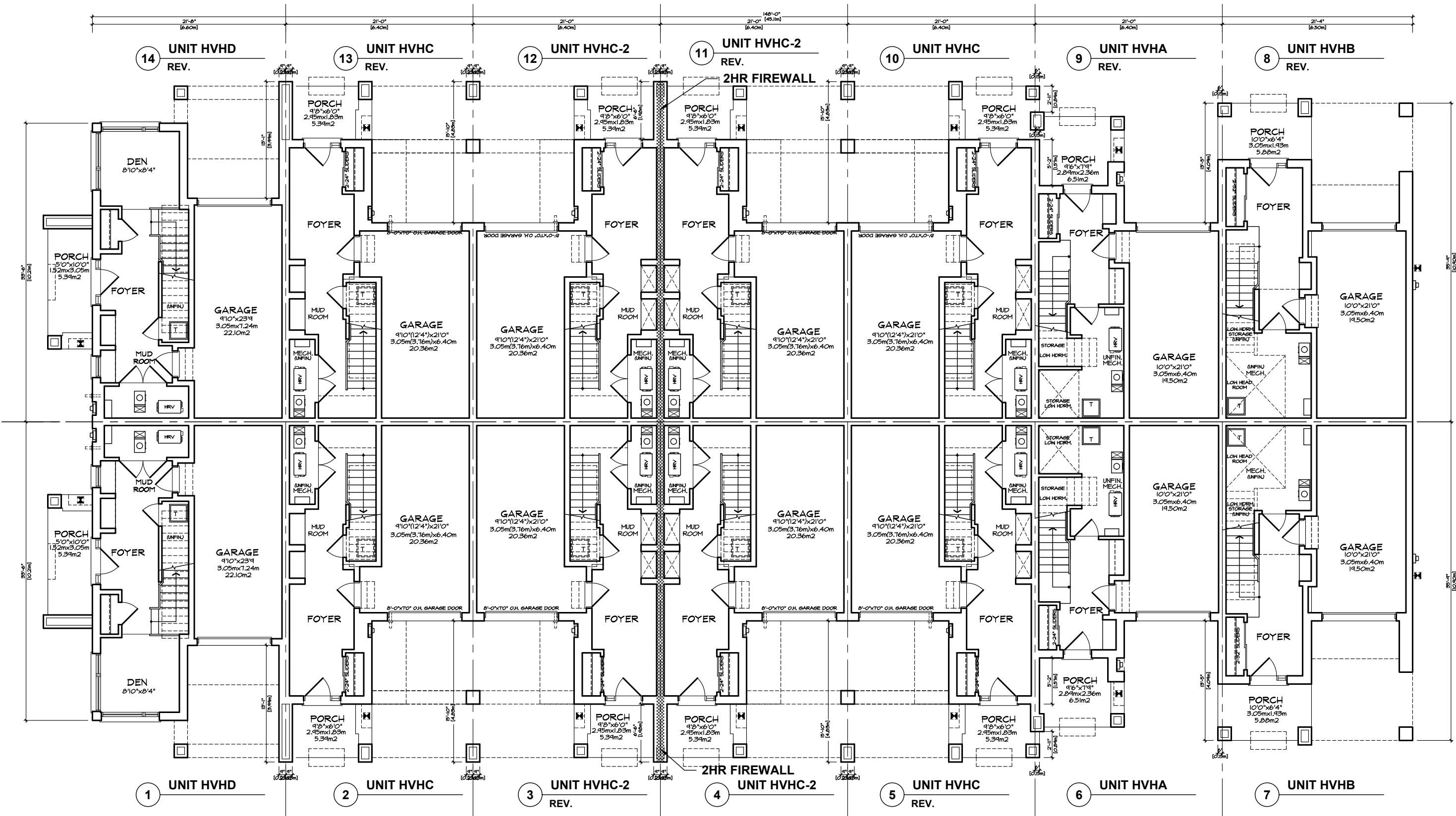
GROUND FLOOR PLAN 'MO' VILLAGE HOMES BLOCK 21
