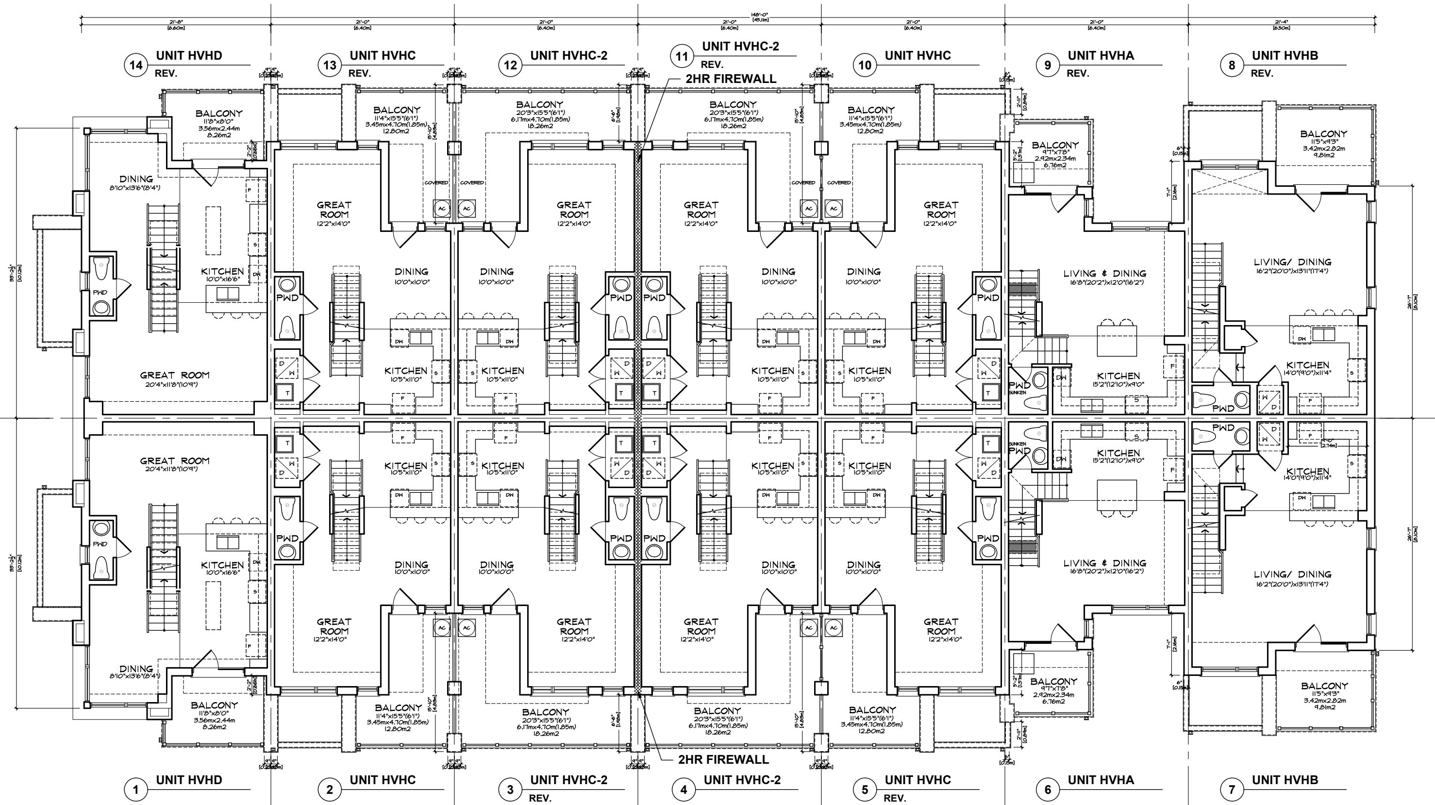
MAIN FLOOR PLAN 'MO' VILLAGE HOMES BLOCK 21
