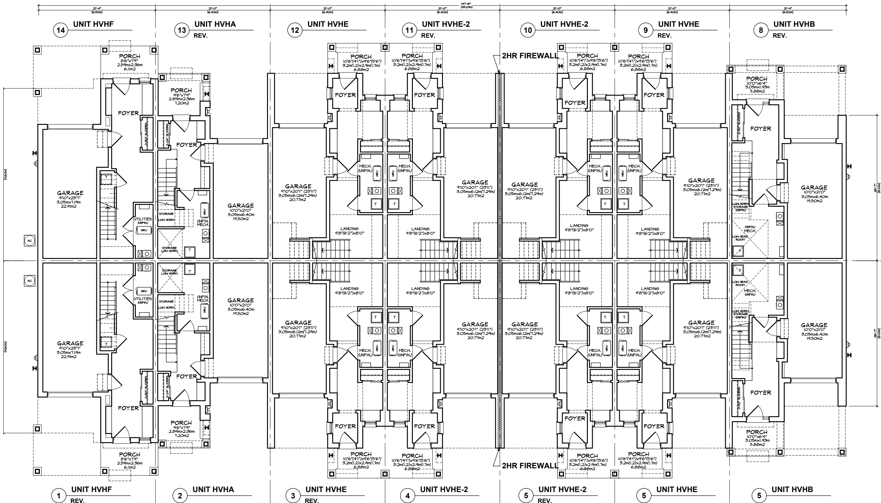
GROUND FLOOR PLAN 'TA' VILLAGE HOMES BLOCK 22
