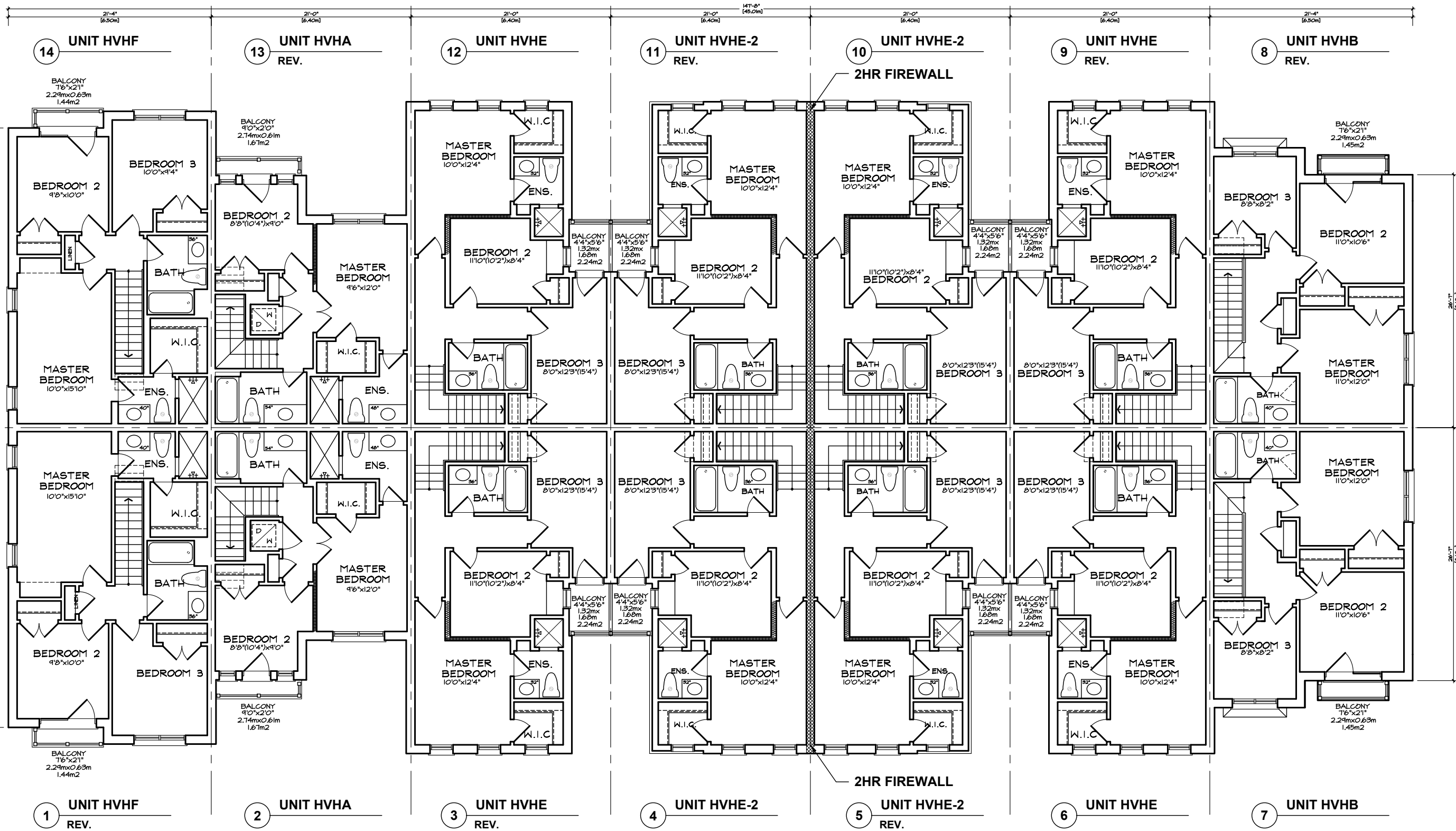
THIRD FLOOR PLAN 'TA' VILLAGE HOMES BLOCK 22
