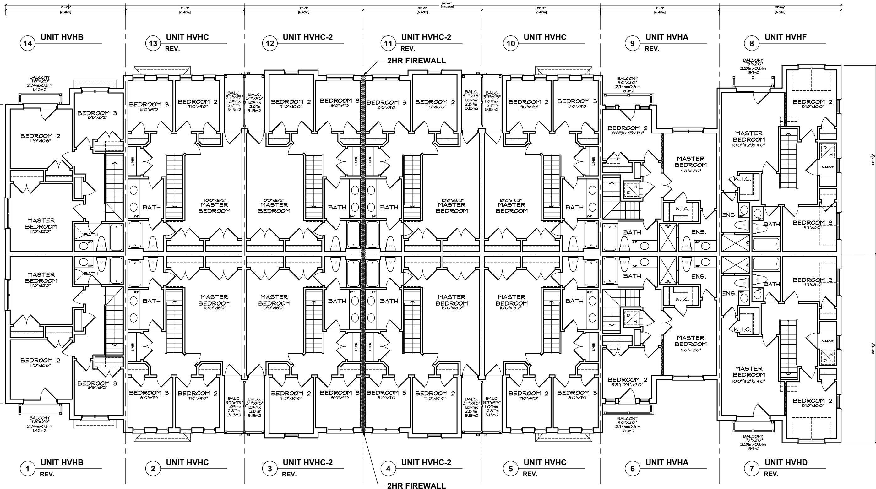
THIRD FLOOR PLAN 'FM' VILLAGE HOMES BLOCK 23
