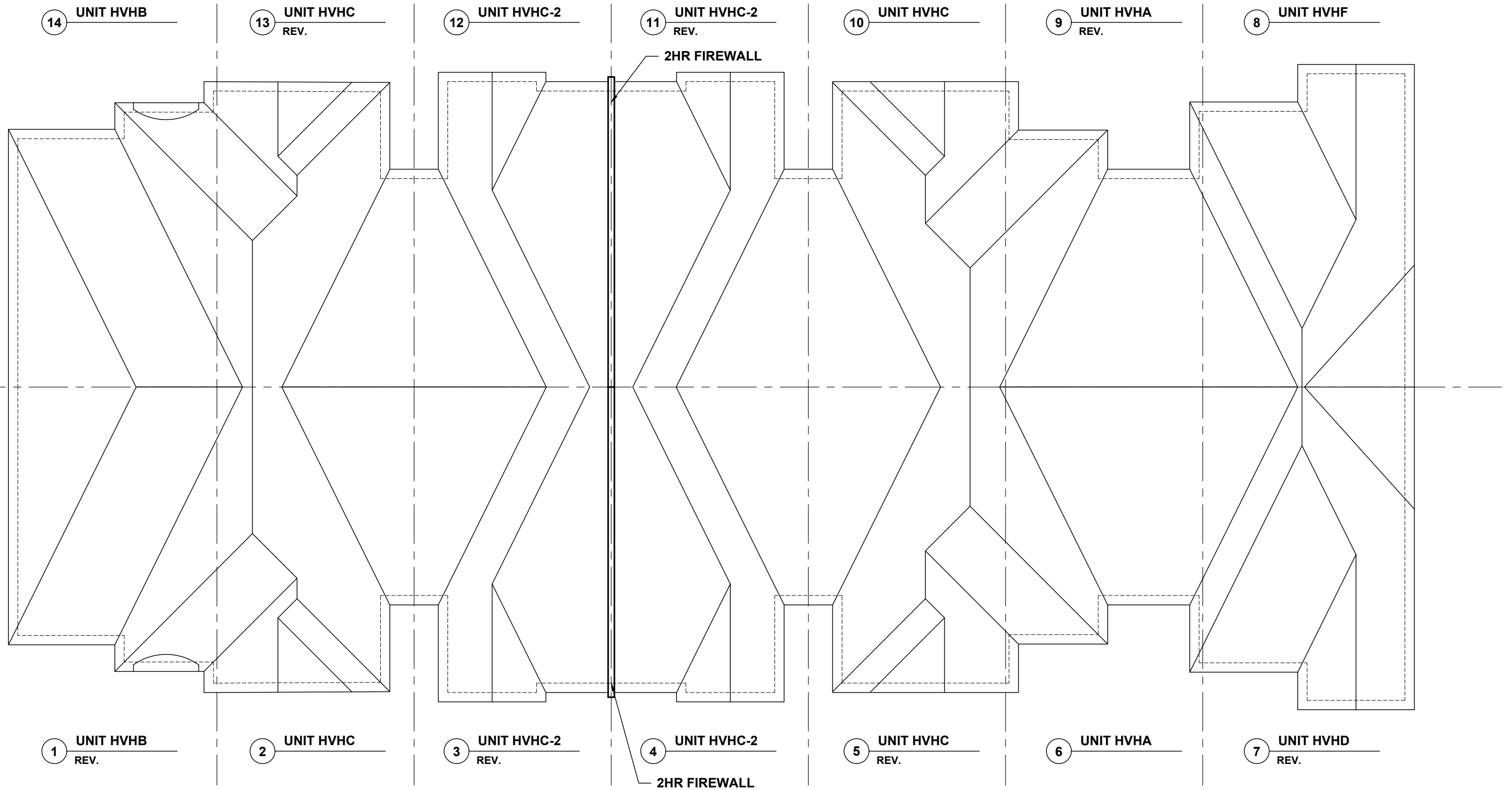
ROOF PLAN 'FM' VILLAGE HOMES BLOCK 23
