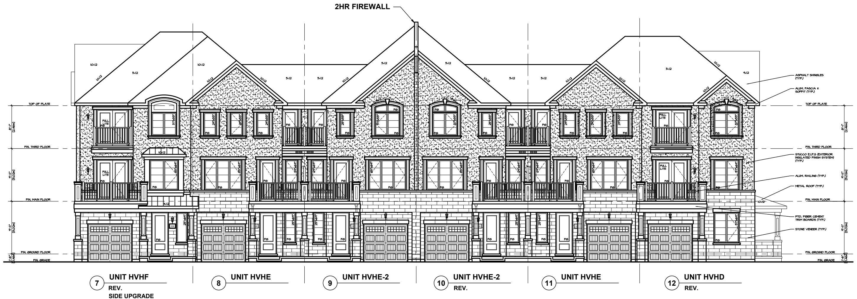
WEST ELEVATION 'FM' VILLAGE HOMES BLOCK 16
