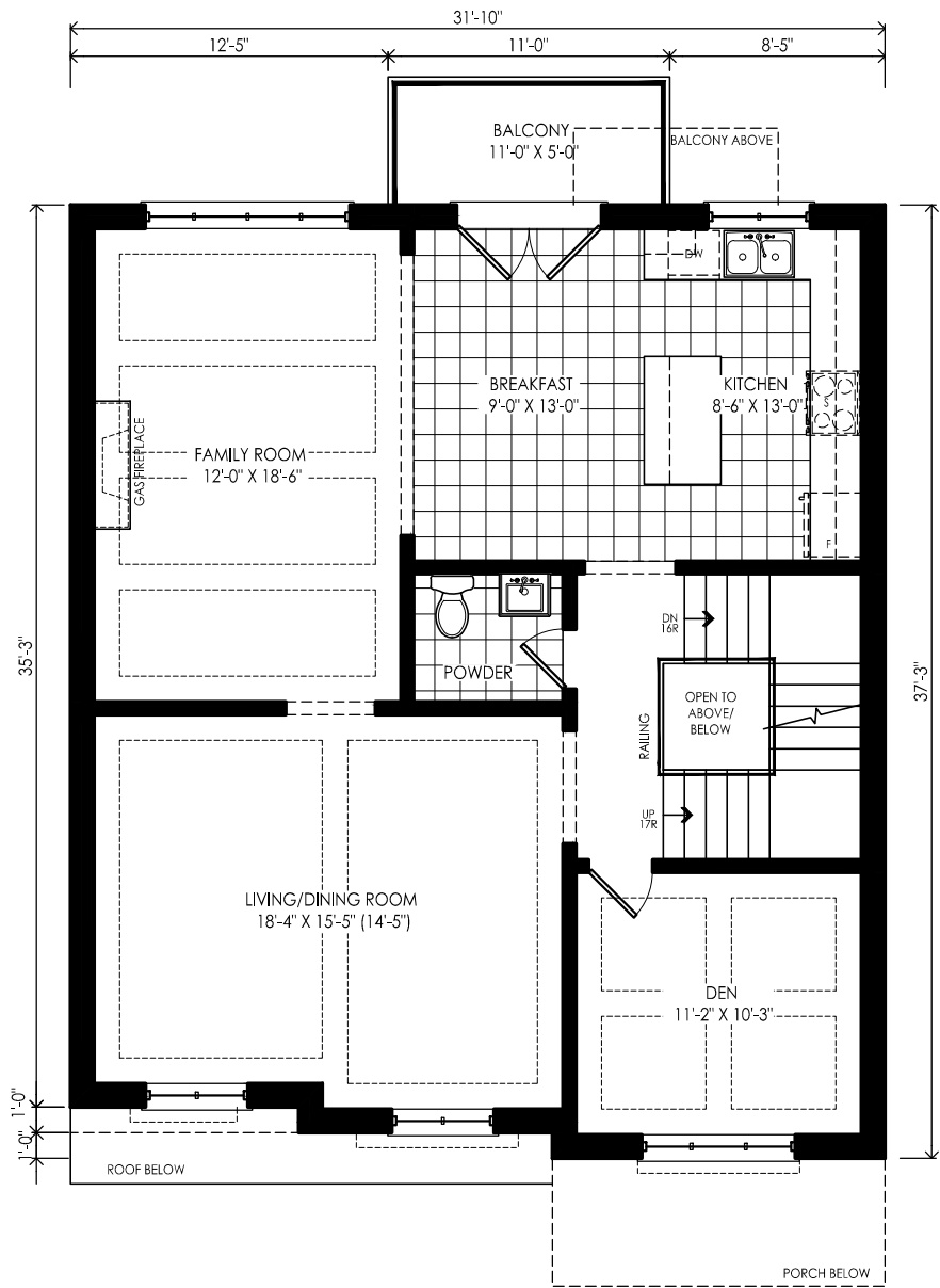
SECOND FLOOR ELEV. 'A' Floor Area: 1158.0 Open To Below: 17.4 Total Area (not incl oib): 1140.6
