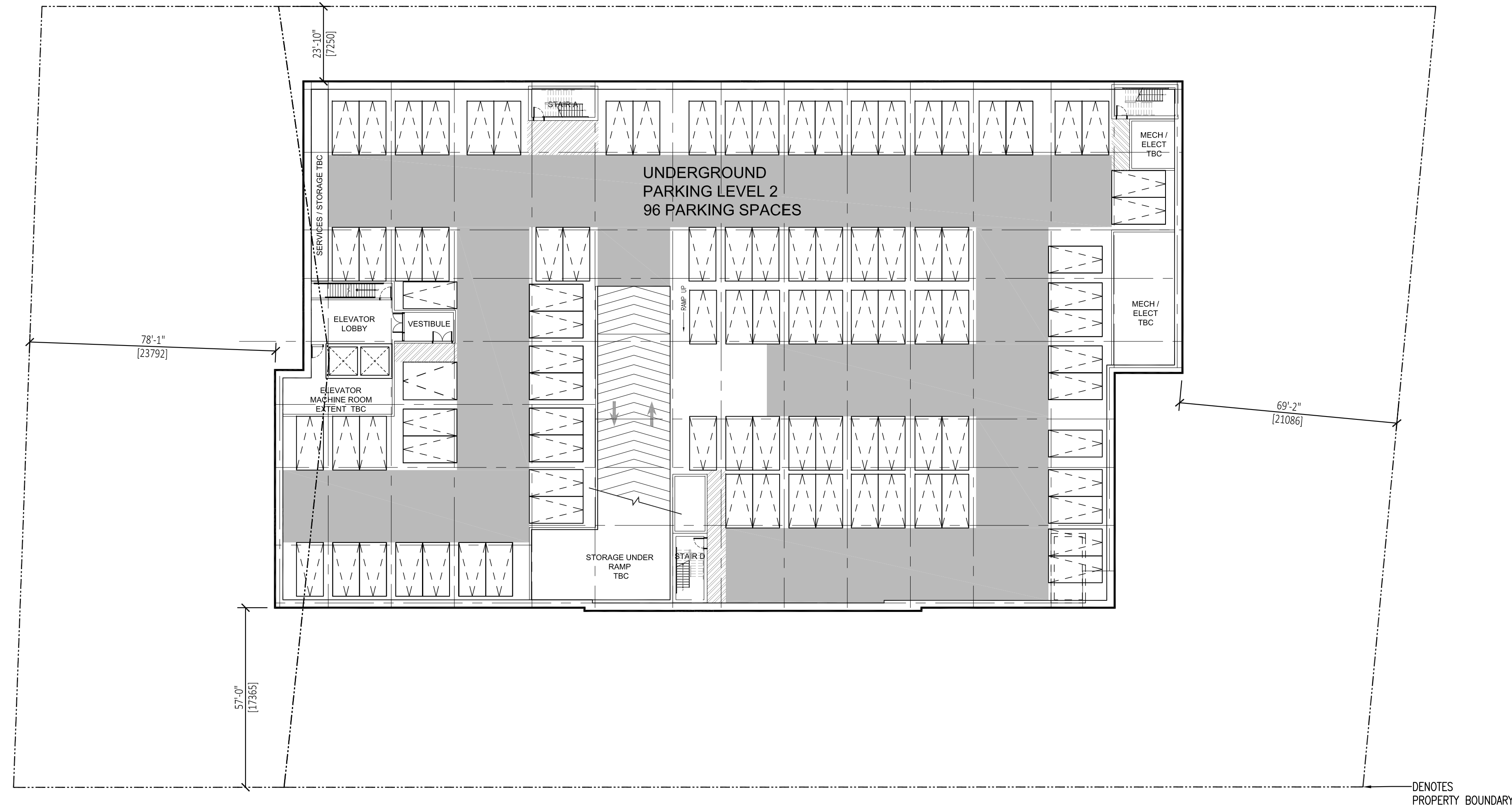
2 UNDERGROUND PARKING LEVEL 2 A-105 SCALE: 1:300
