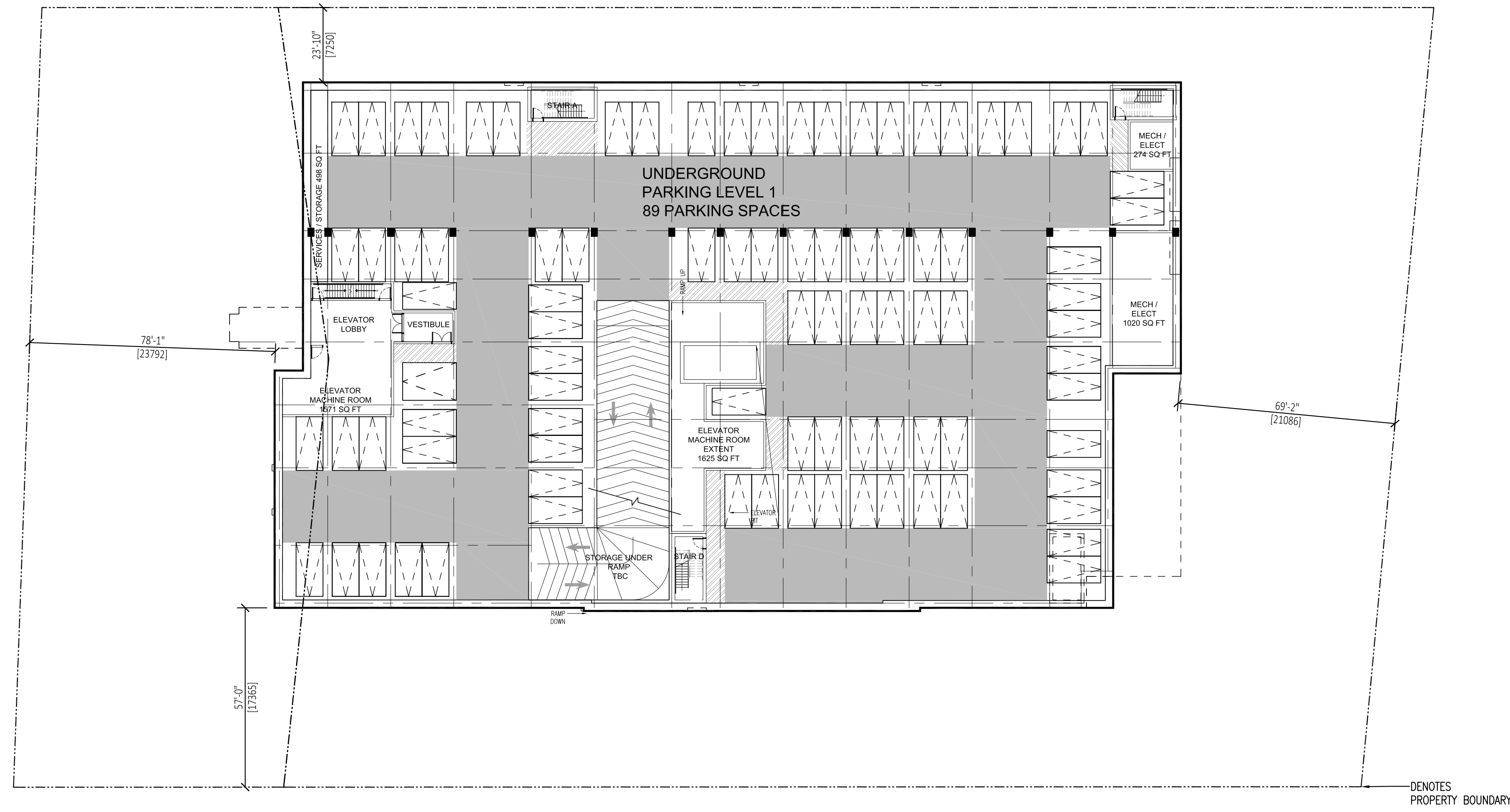
1 UNDERGROUND PARKING LEVEL 1 A-105 SCALE: 1:300
