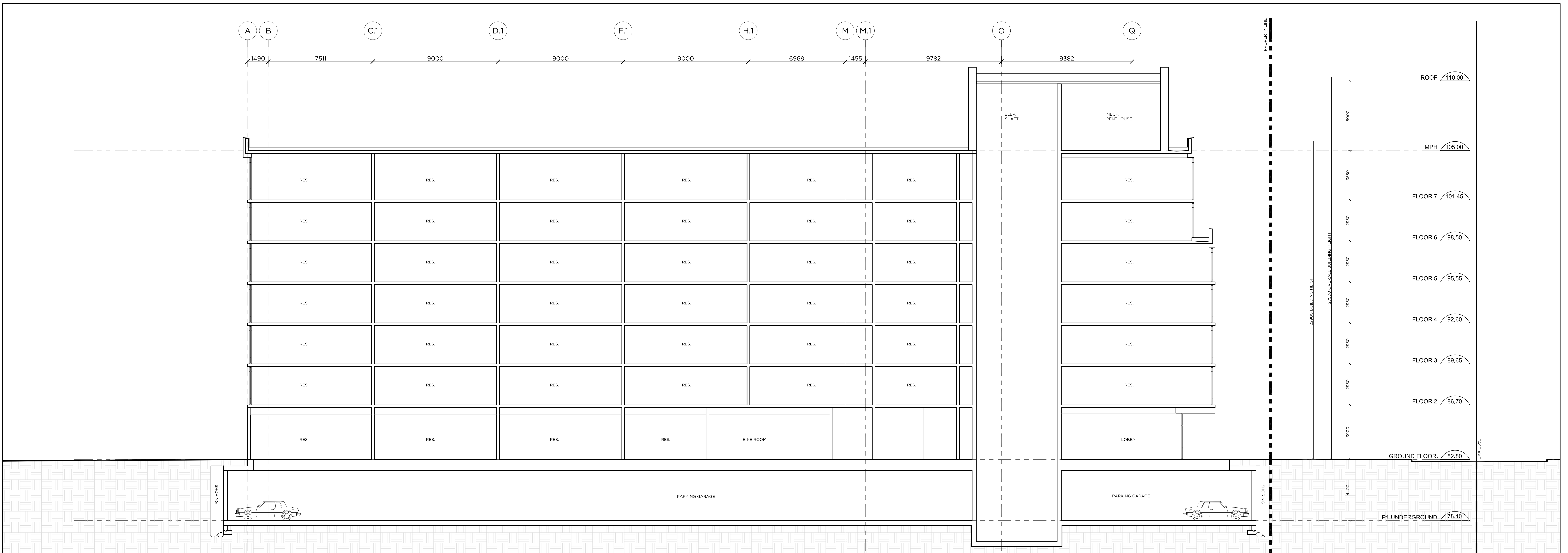
1 BUILDING SECTION SCALE 1/8" = 1'-0"
