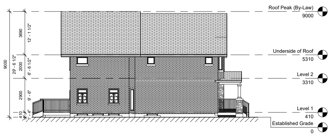
2 South Elevation 1 : 100
