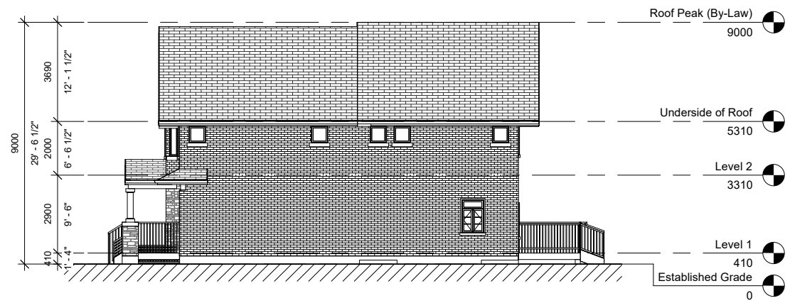
1 North Elevation 1 : 100
