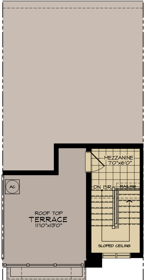
MEZZANINE PLAN
