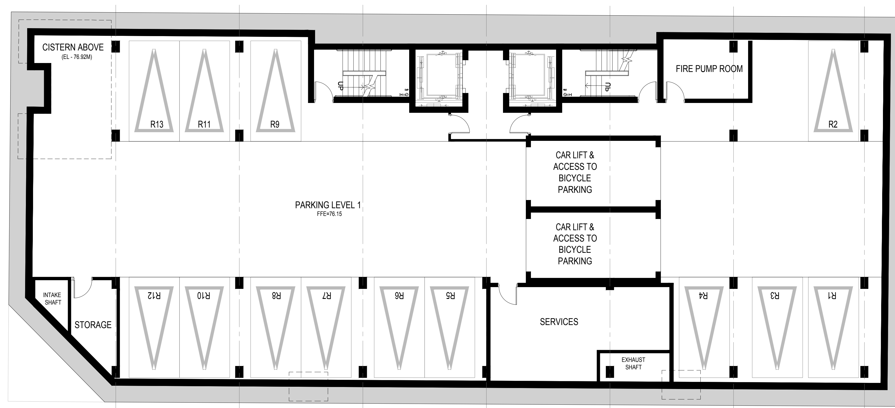
P1 PARKING 13 CARS
