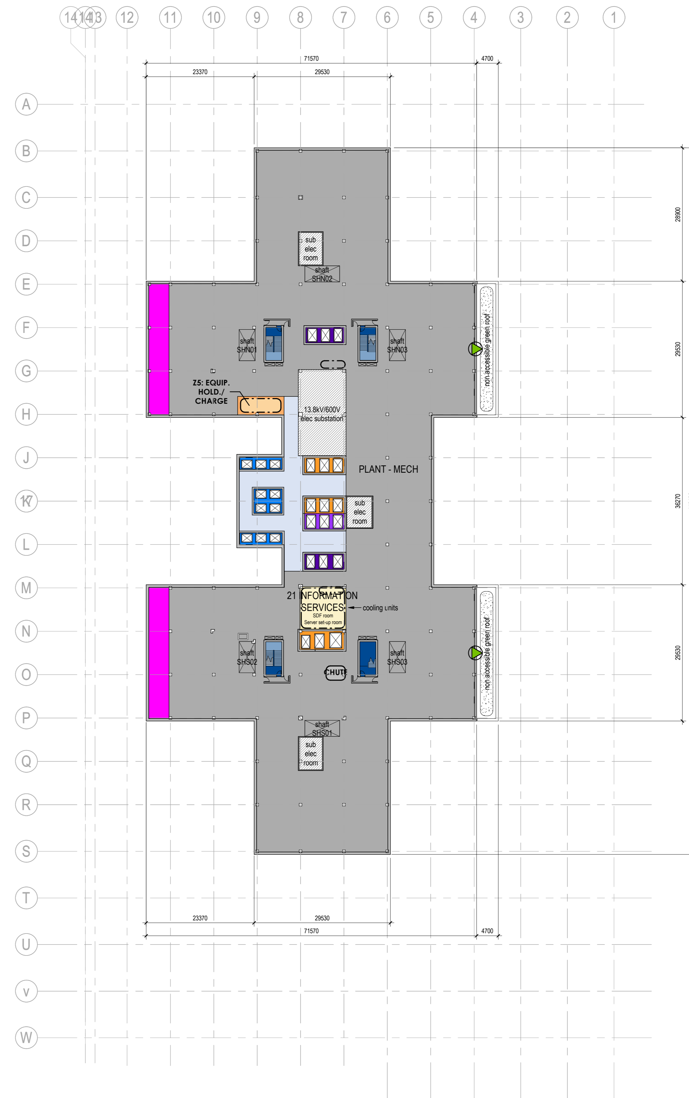
2 DEPARTMENTAL ZONE STUDY - LEVEL 15 M&E PLANT A-204 1:500
