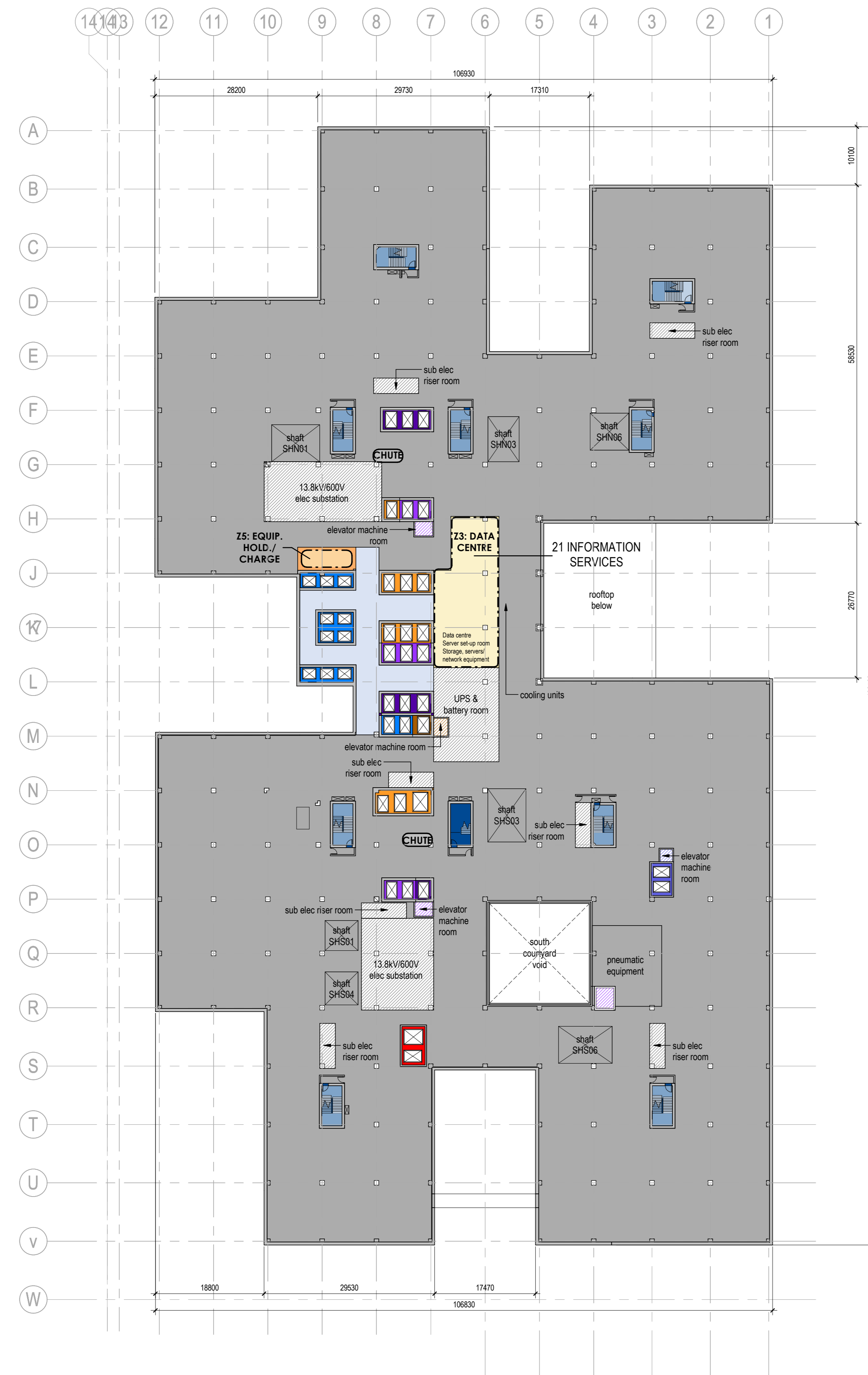
1 DEPARTMENTAL ZONE STUDY - LEVEL 7 M&E PLANT A-204 1:500
