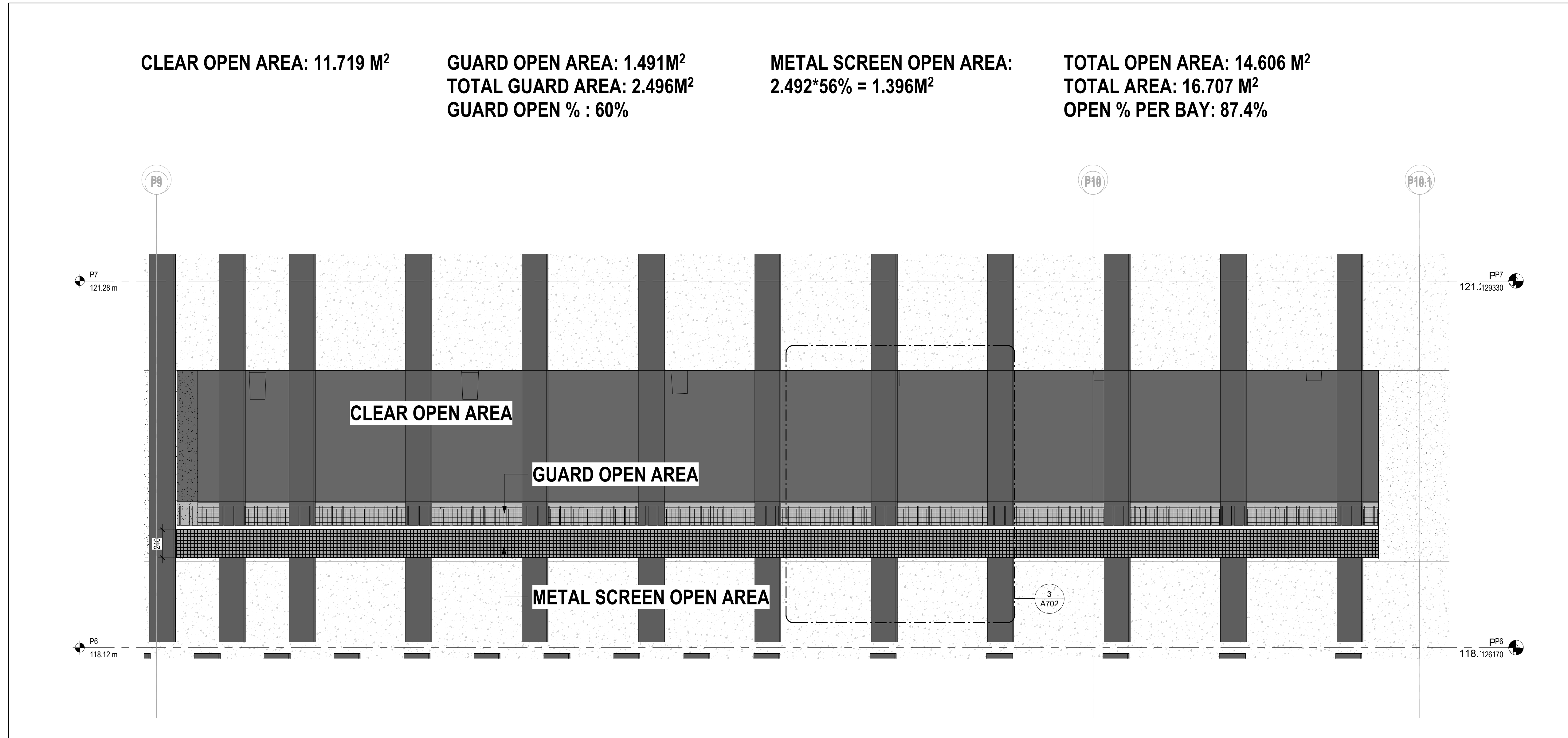
SECTION DETAIL - TYP BAY OPENING SCALE: 1:20
