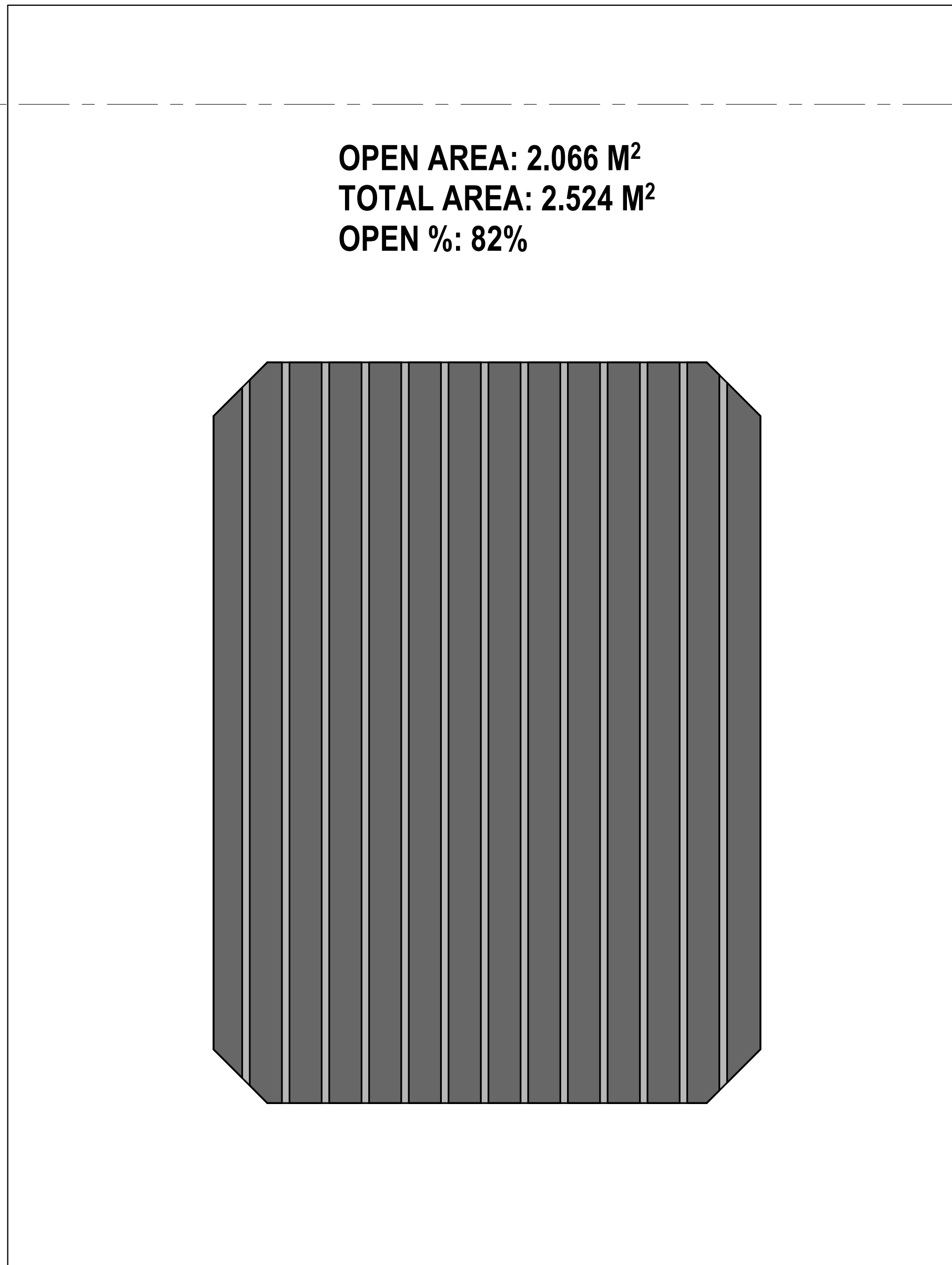
SECTION DETAIL - TYP COLUMN WALL OPENING SCALE: 1:10
