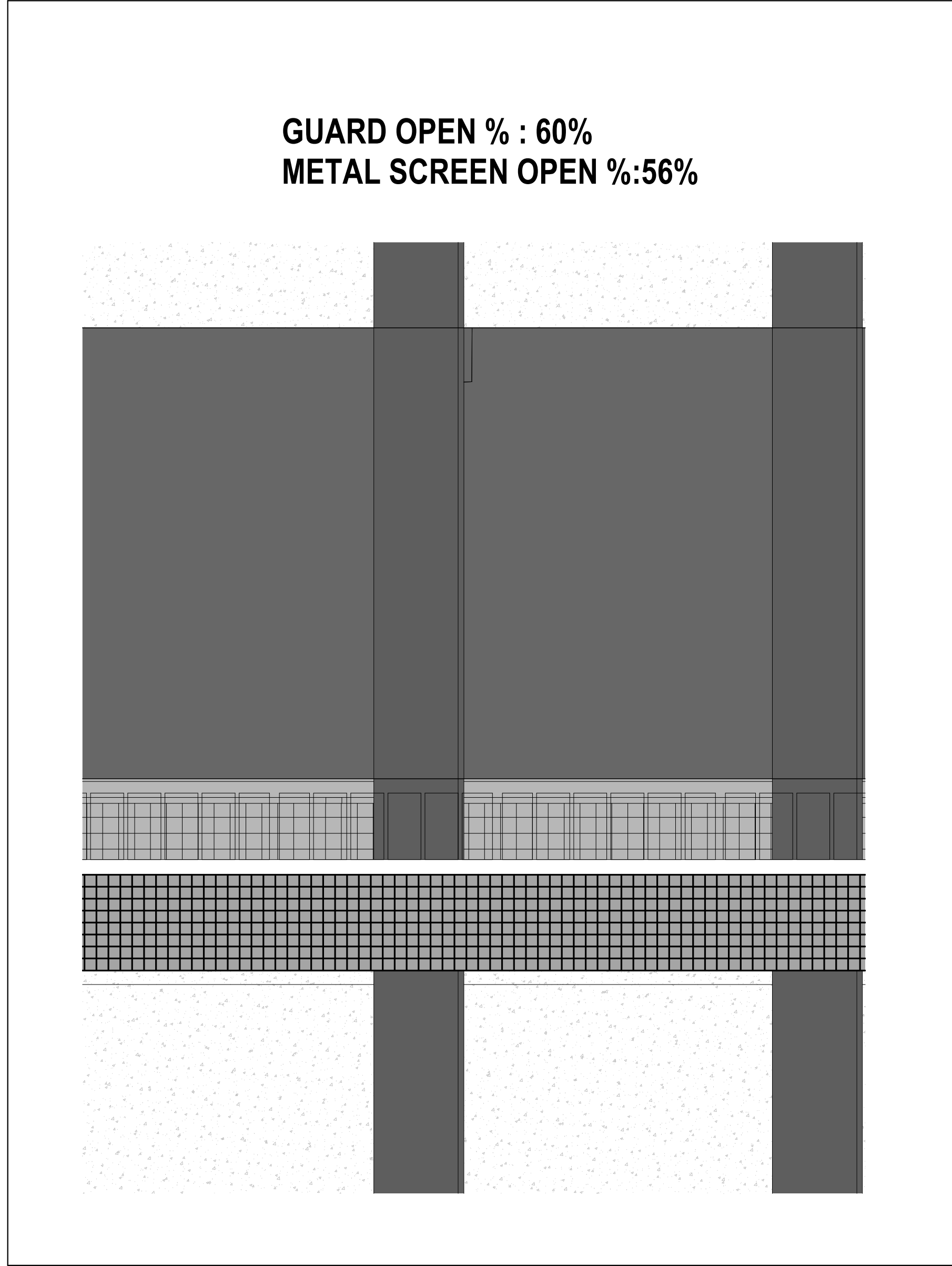
ENLARGED SECTION DETAIL - TYP BAY OPENING SCALE: 1:10
