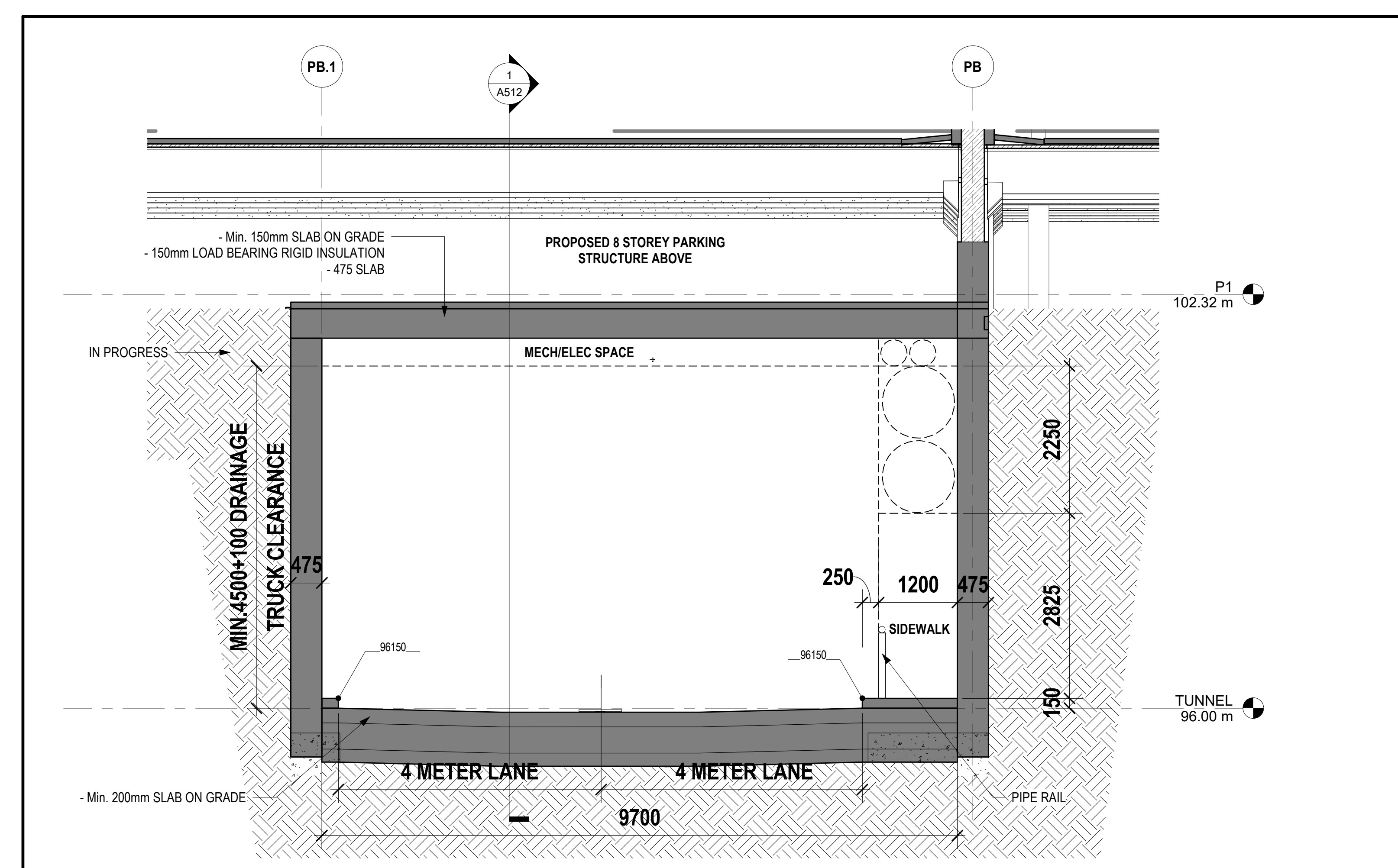
ENLARGED SECTION - TUNNEL - NORTH/SOUTH UNDER DOUBLE TEE STRUCTURE SCALE: 1:50 AS13
