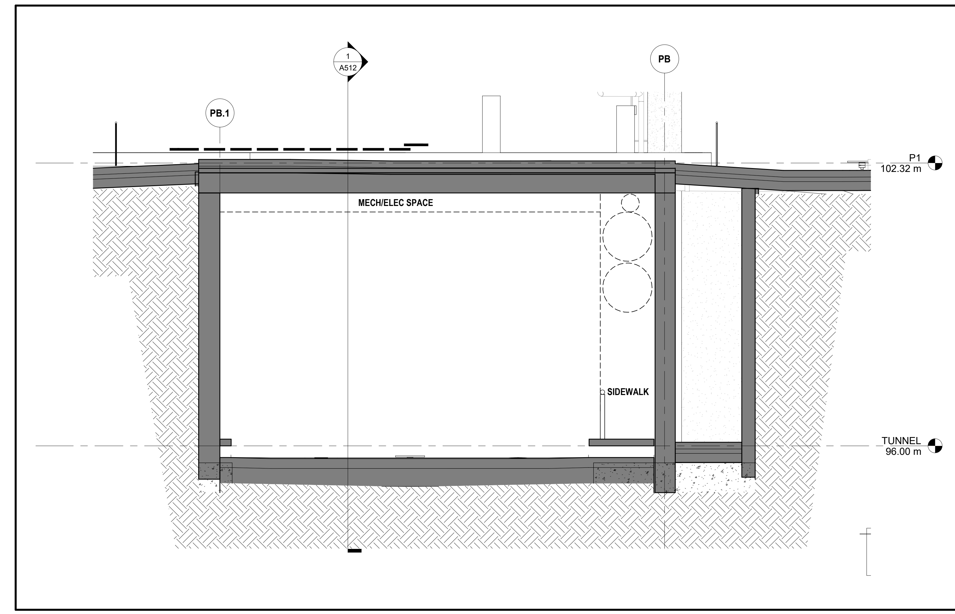
ENLARGED SECTION - TUNNEL - NORTH/SOUTH AT DRIVE WAY SCALE: 1:50 AS13
