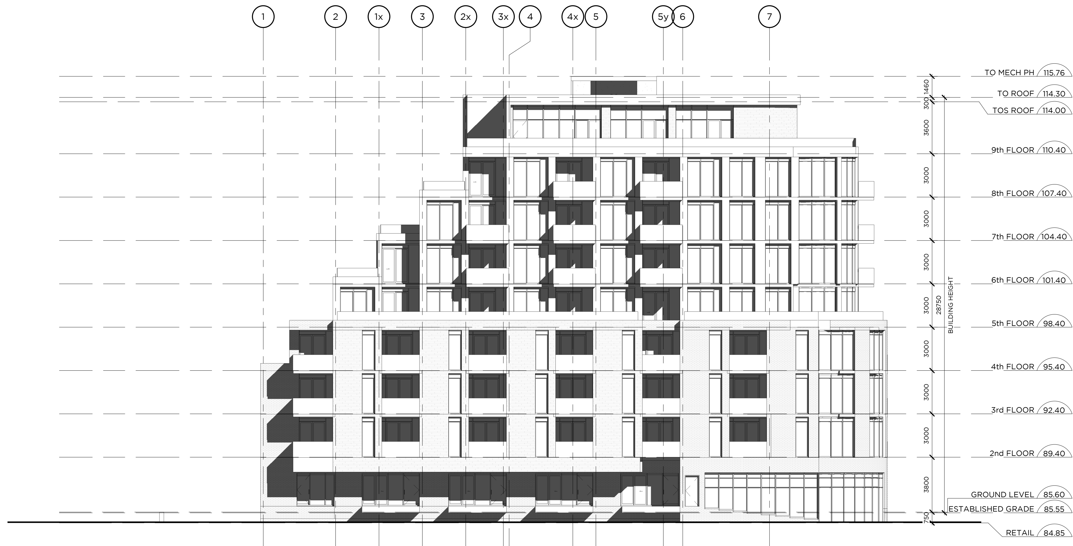
1 SOUTH EAST ELEVATION A401/1:150
