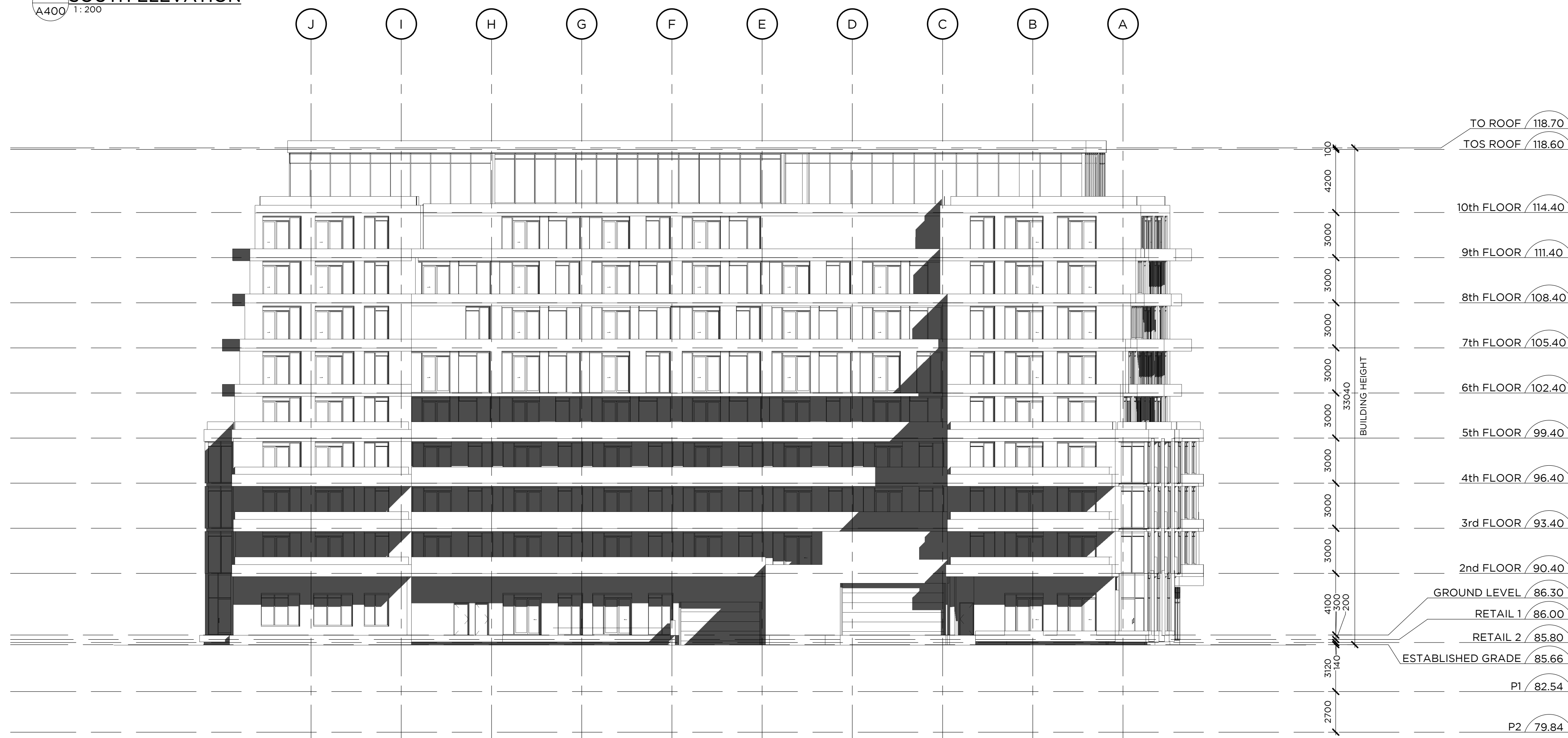
1 SOUTH ELEVATION A400 1:200
