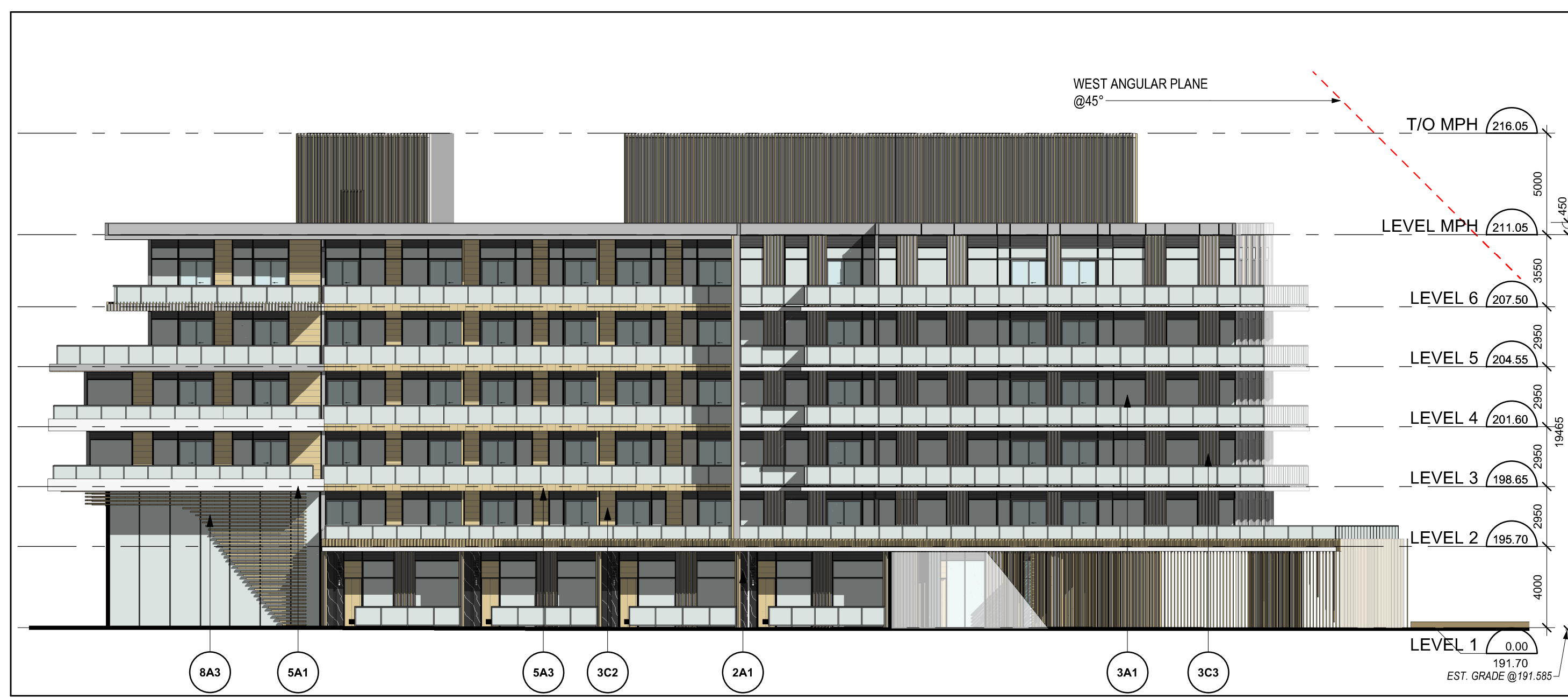
North Elevation 4 1 : 200 A400
