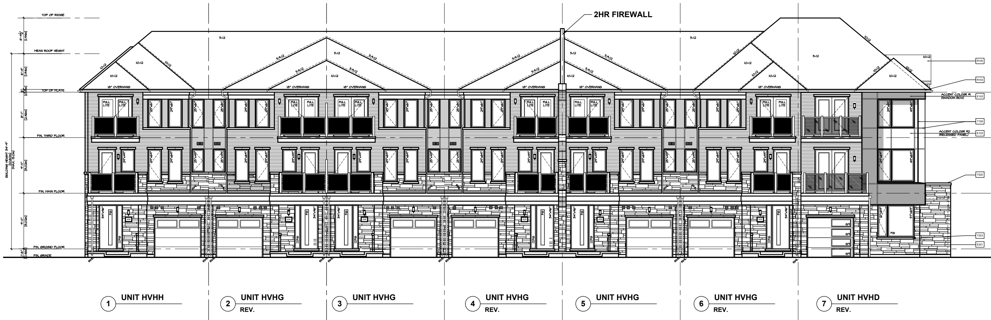
EAST ELEVATION 'MO' VILLAGE HOMES BLOCK 23
