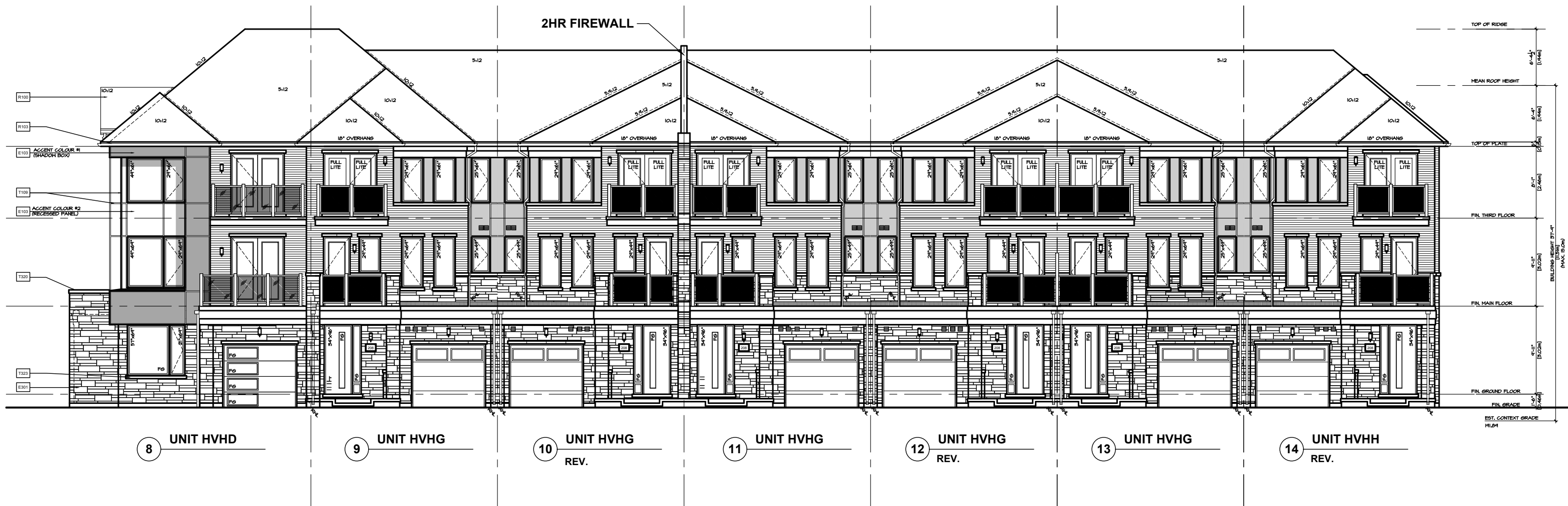
WEST ELEVATION 'MO' VILLAGE HOMES BLOCK 23
