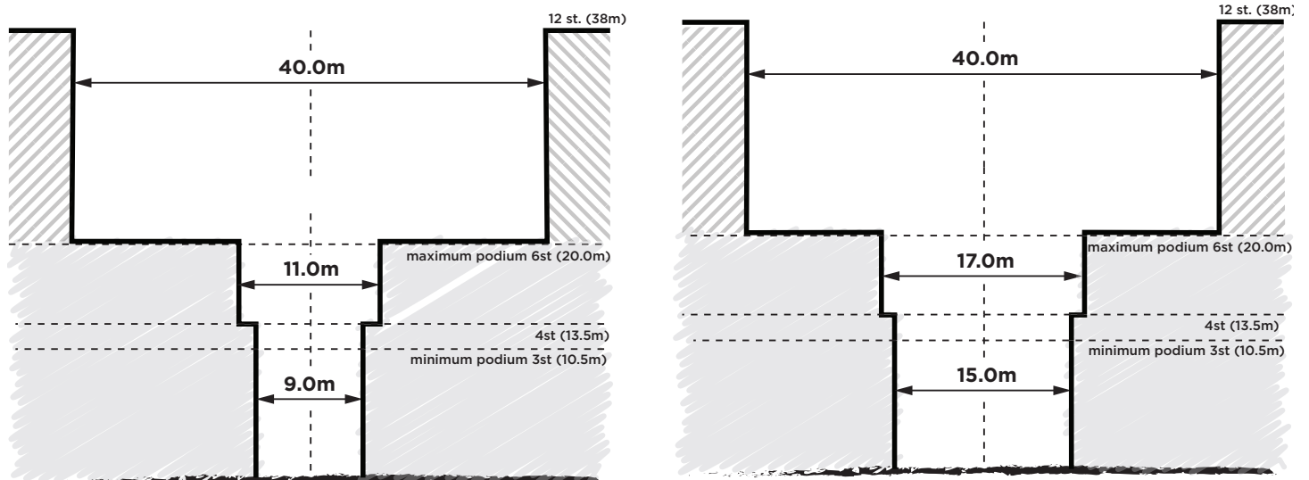
Figure 8.9 Proposed separation between Tall buildings on same or adjacent sites. (Left) Side Wall to Side Wall, with or without fenestration (Right) Front Wall to Front Wall, Front Wall to Side Wall, with or without fenestration
