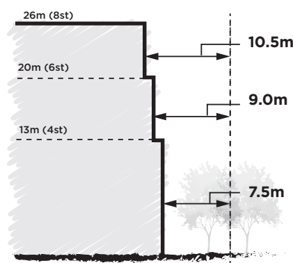
Figure 8.5 Proposed Setbacks
