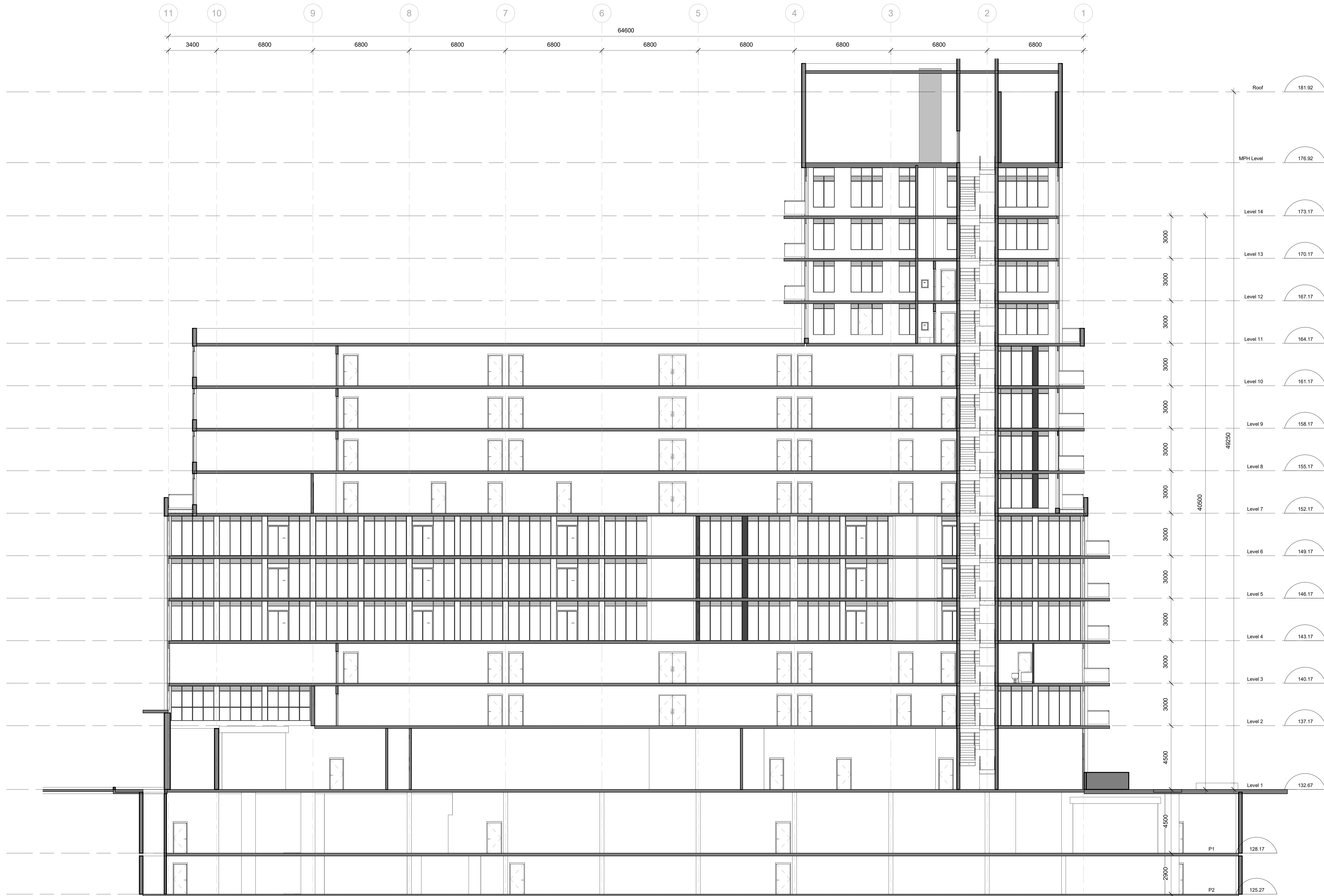
1 Longitudinal Building Section 1 : 100
