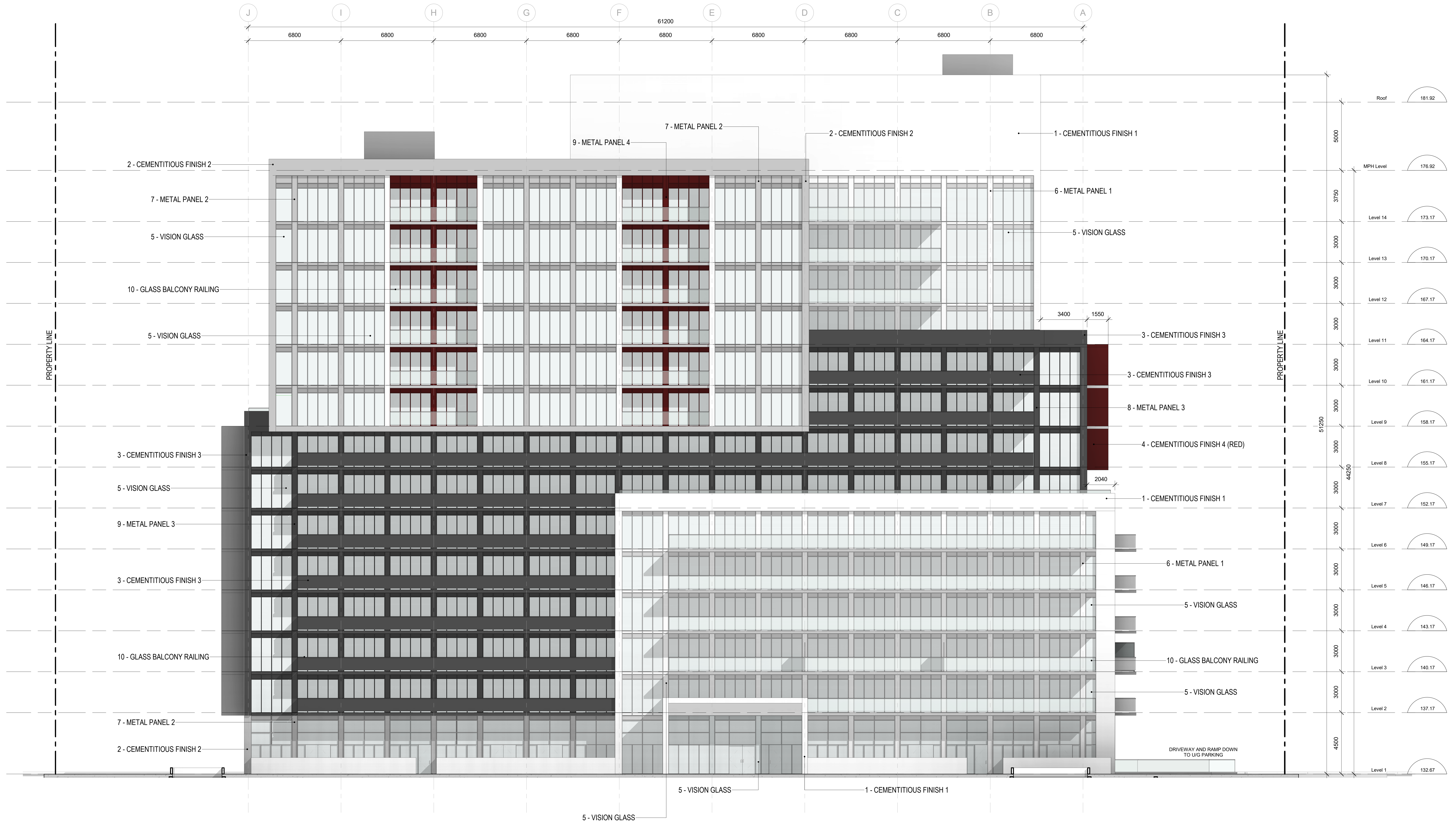
1 North Elevation 1 : 100
