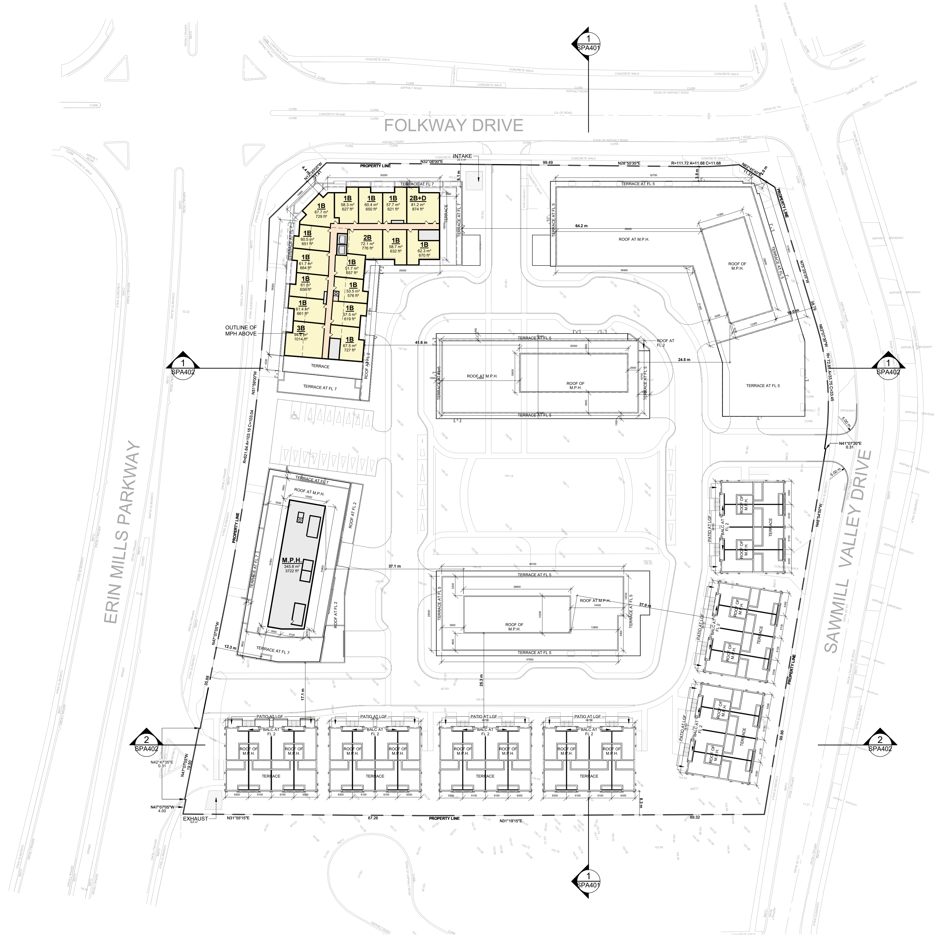
1 FLOOR 09-10 1:500
