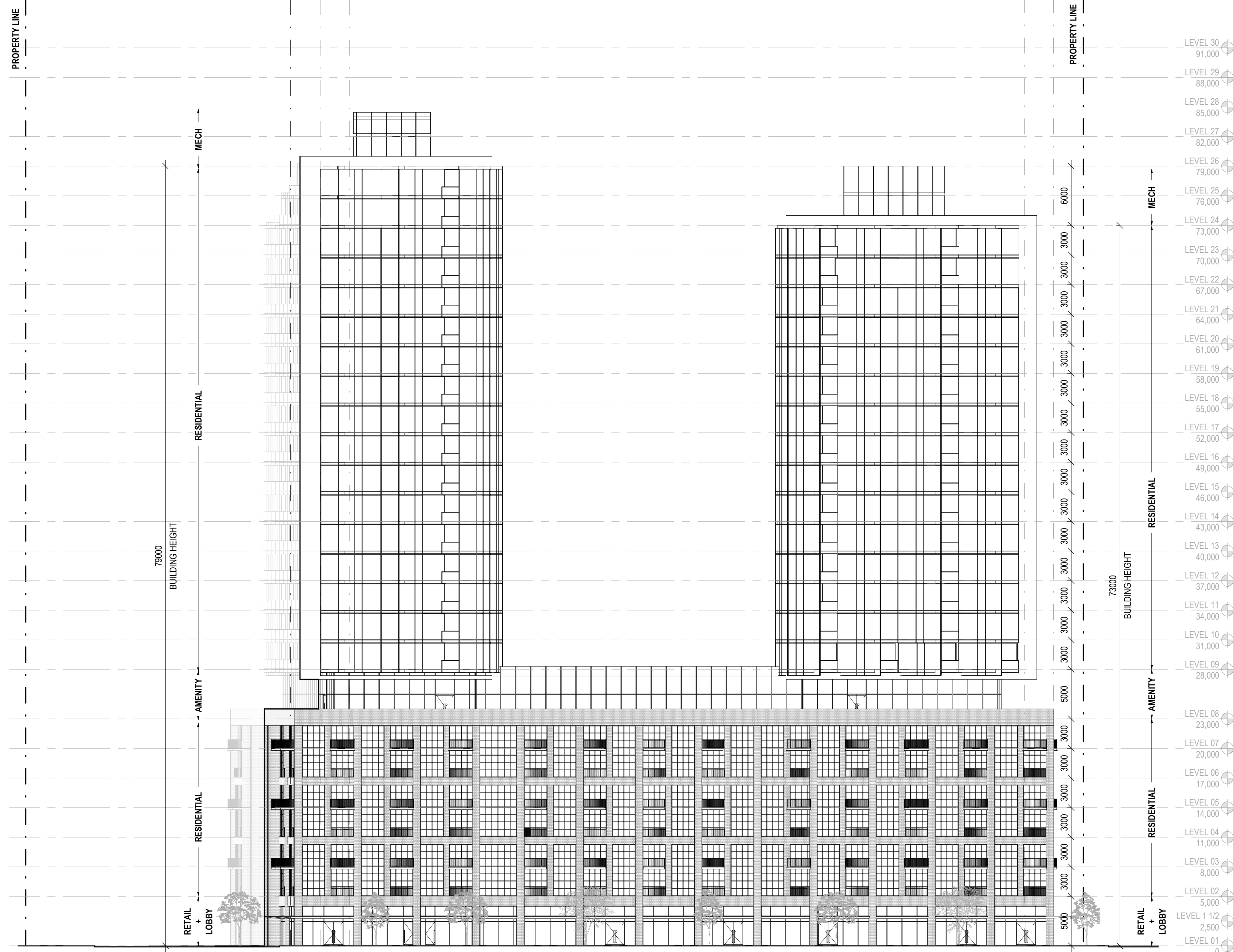
4 SITE ELEVATION - CENTRAL STREET E SCALE: 1 : 250
