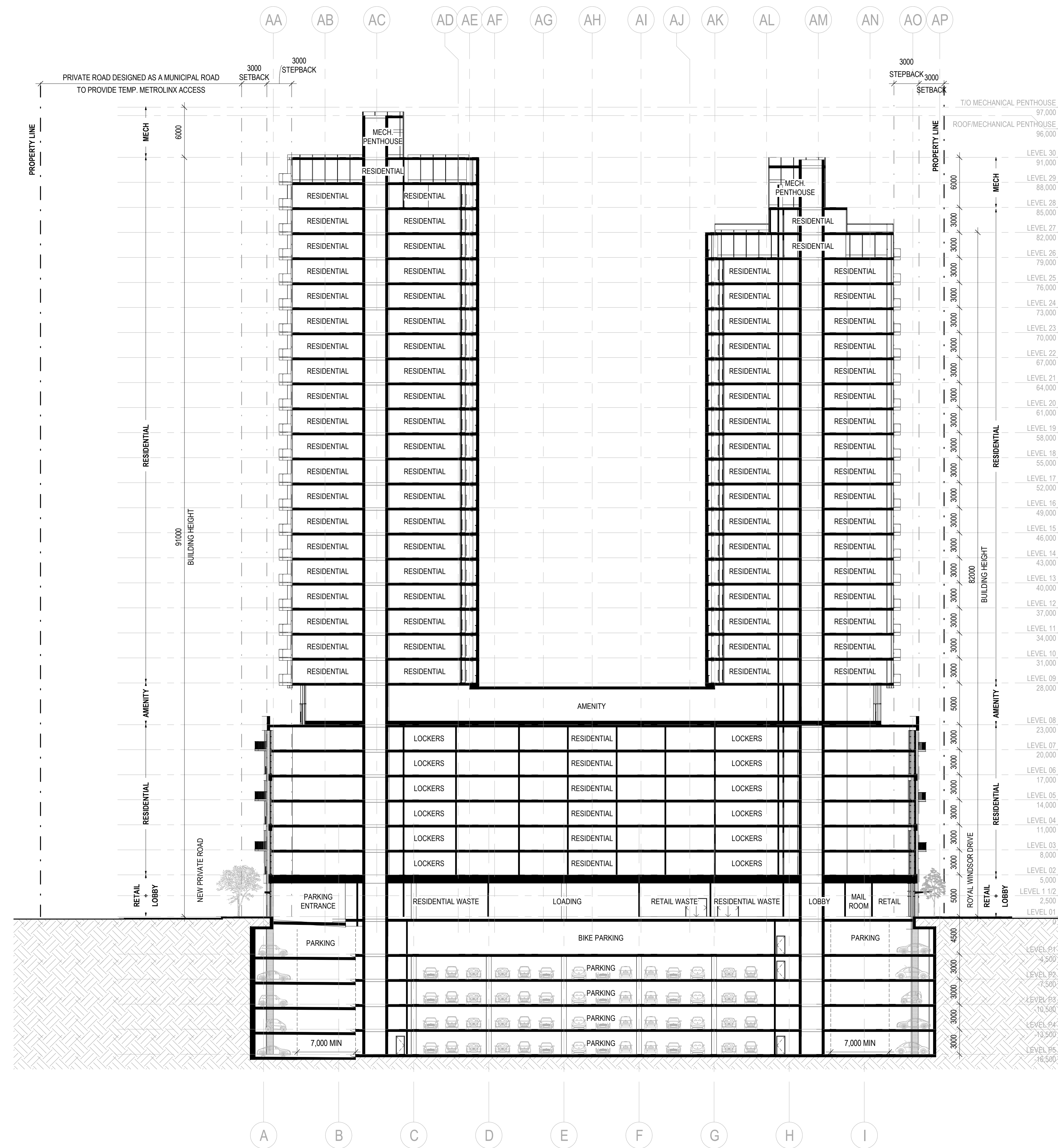
1 BUILDING SECTION - NS WEST SIDE SCALE: 1/250
