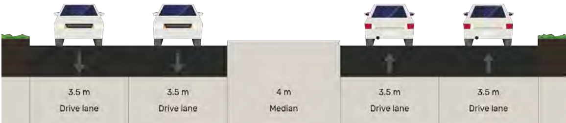
Figure 10 - Existing cross section (centre section, with median)
