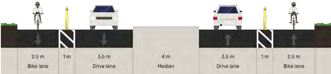
Figure 11 - Proposed cross section (centre section)
