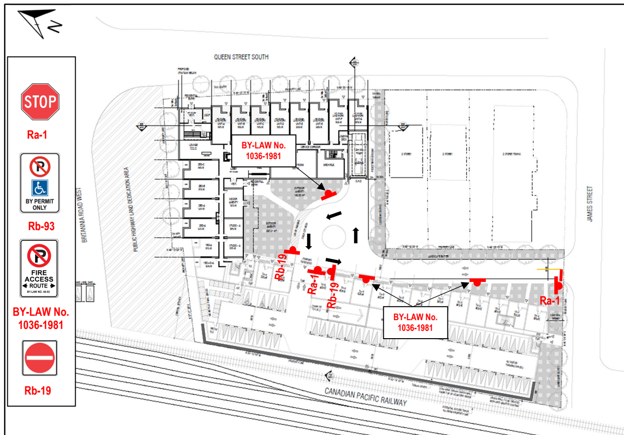
Figure 13 – Preliminary Proposed Pavement Marking and Signage Plan
