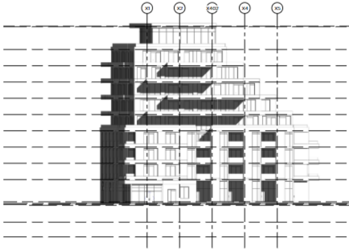
1 EAST ELEVATION K410
