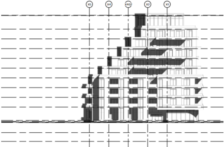
1 SOUTH ELEVATION K410
