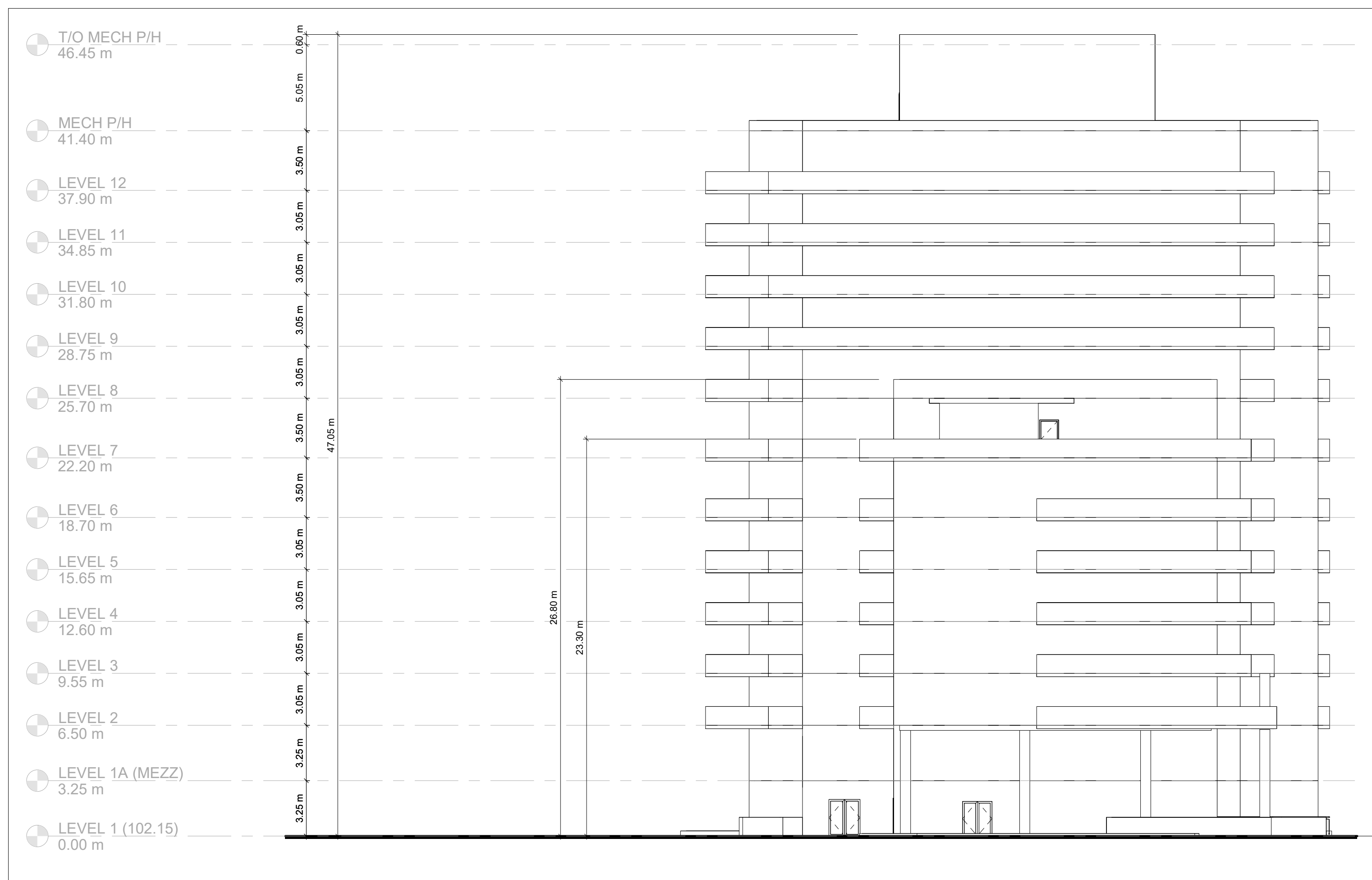
1 EAST ELEVATION 1 : 200
