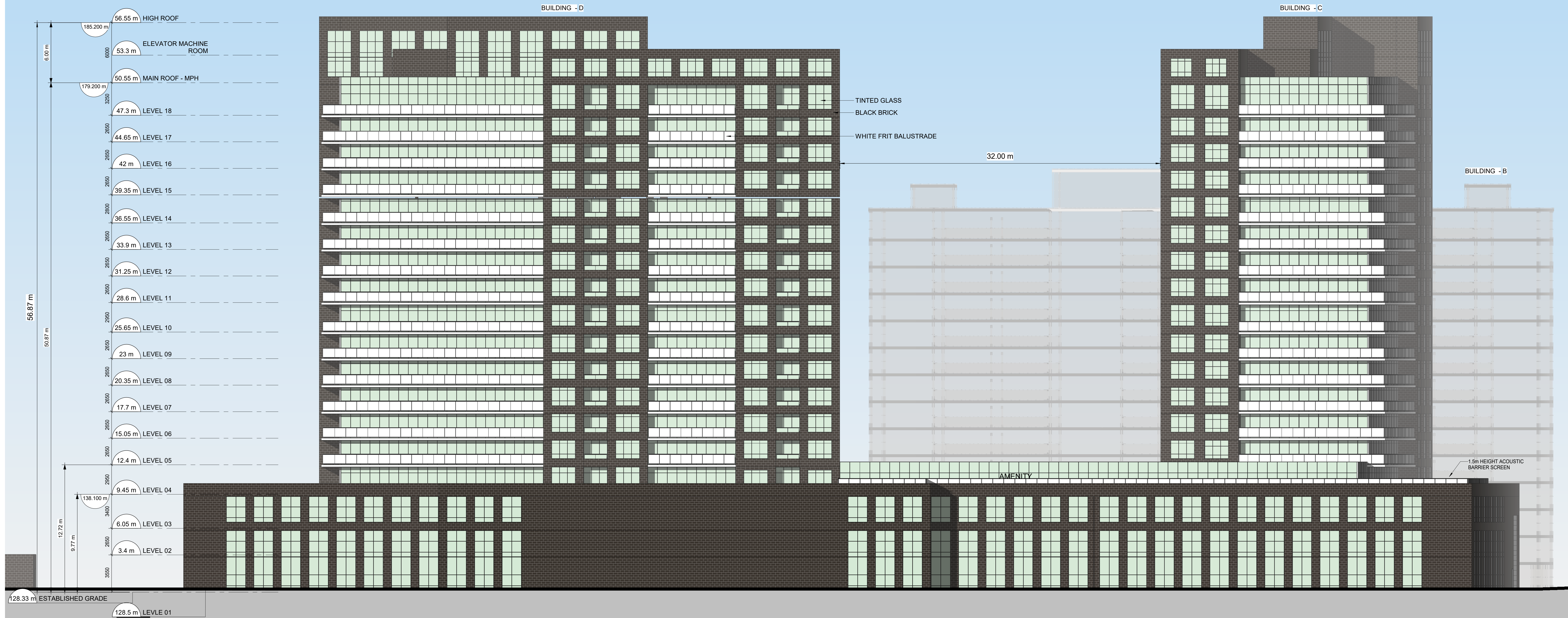
1 SOUTH ELEVATION Scale: 1:150
